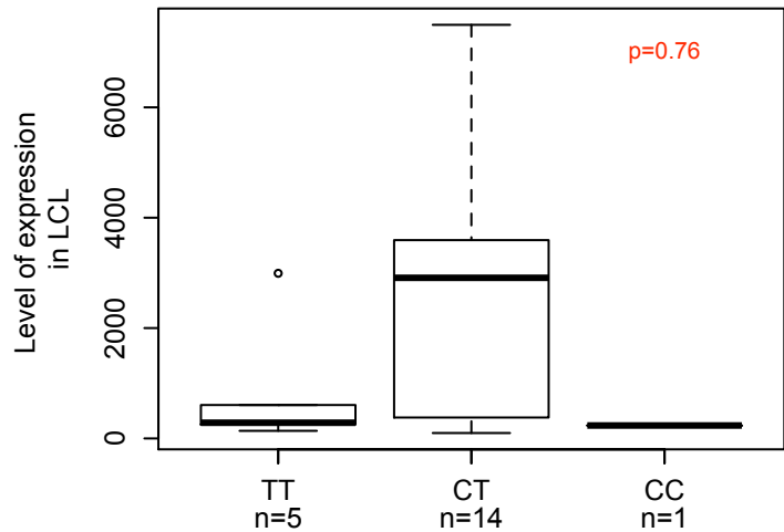
BRCA1
