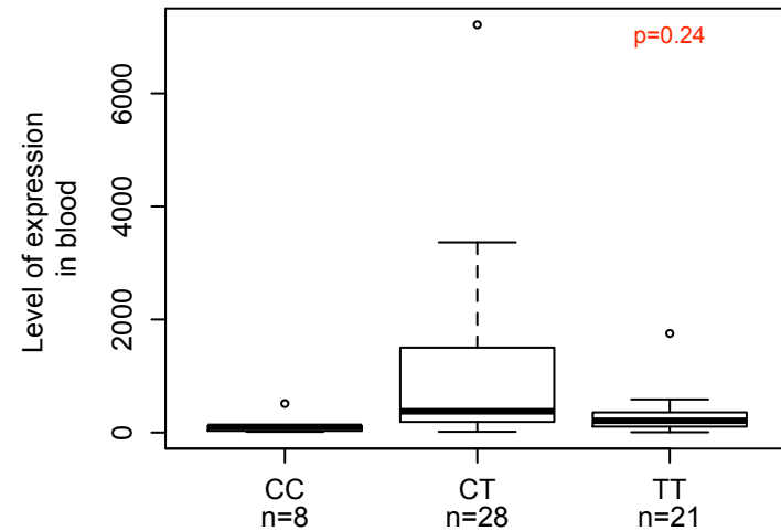
NBS1
