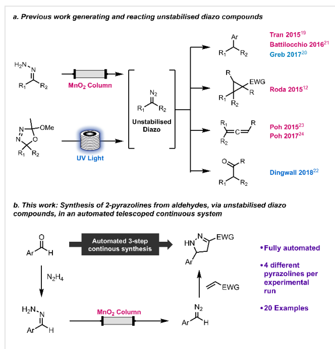
Scheme 1 Previous work handling unstabilised diazo compounds (a) and this work on the multi-step synthesis of 2-pyrazolines from aldehydes (b).
