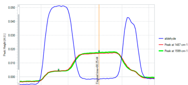
Figure 2 Consumption of aldehyde starting material when hydrazine reagent is injected, and identification of peaks at 1487 cm -1 and 1599 cm -1 indicative of the presence of the intermediate.
