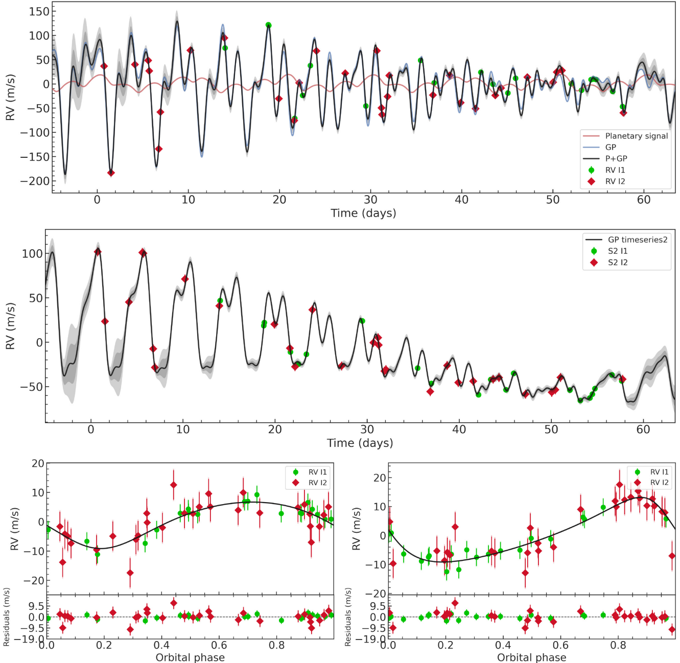
Figure 4. S_1 and S_2 time-series described in Section 5.2. Top panel: The green (instrument I_1 ) and red markers (instrument I_2 ) in each panel represent the synthetic measurements with inferred offsets extracted. Solid dark line and shadow regions are as in Fig. 3. The RV-like time-series also included the RV model for the two planets (red line). Bottom panel: Synthetic RV-like data folded on the orbital period of each injected planet following the subtraction of the systemic velocities, GP signal, and the other planet. The plots also show the inferred RV model for each planet (solid black line). These plots were generated automatically by pyaneti .
