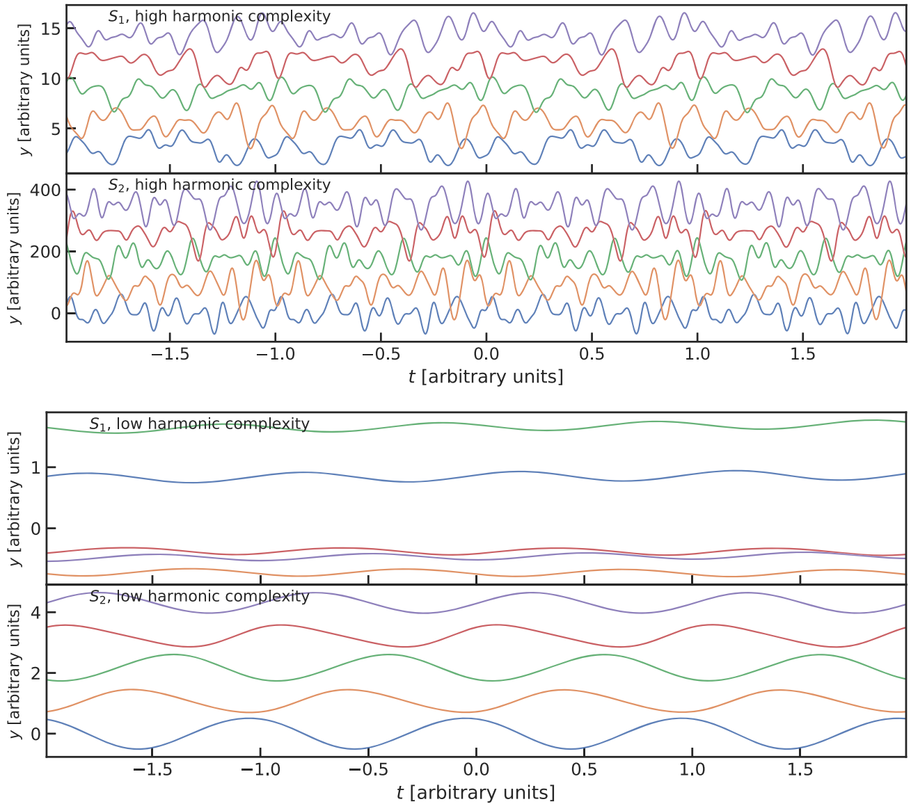
Figure 2. Example of samples from a multidimensional GP (two dimensions in this case) created with a QP kernel with P_{\text{GP}} = 1 , \lambda_e = 10 and high ( \lambda_p = 0.1 , top panel) and low \lambda_p = 10 , lower panel) levels of harmonic complexity. Each panel shows two subplots with samples of S_1 and S_2 time-series (See equation 11). Corresponding S_1 and S_2 draws from the same sample are shown with the same colour.
