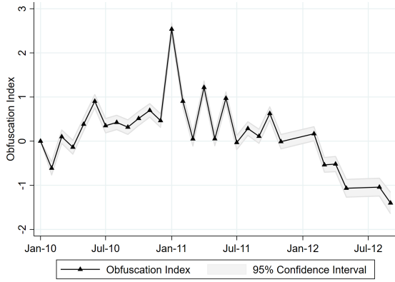
Figure 10: Obfuscation index
