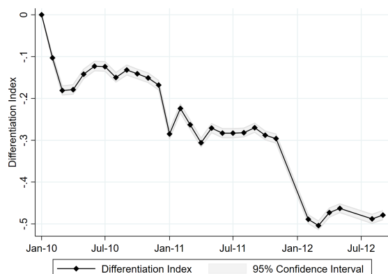
Figure 8: Differentiation index
