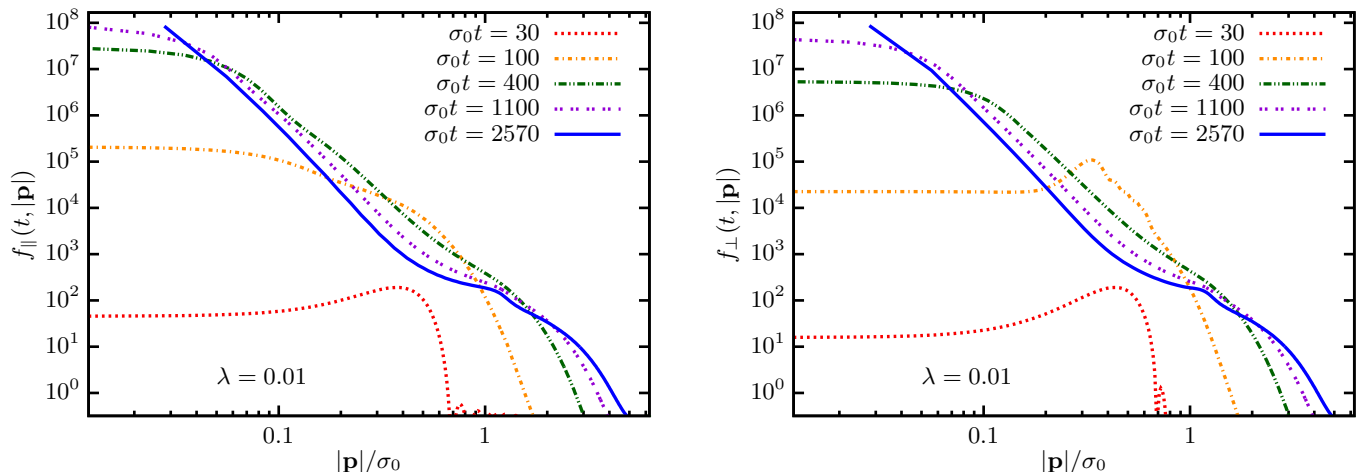
Figure 9. Longitudinal ( \parallel , left ) and transverse ( \perp , right ) occupation number distributions for macroscopic field initial conditions with \lambda = 0.01 at different times showing the emergence of a dual cascade picture.
