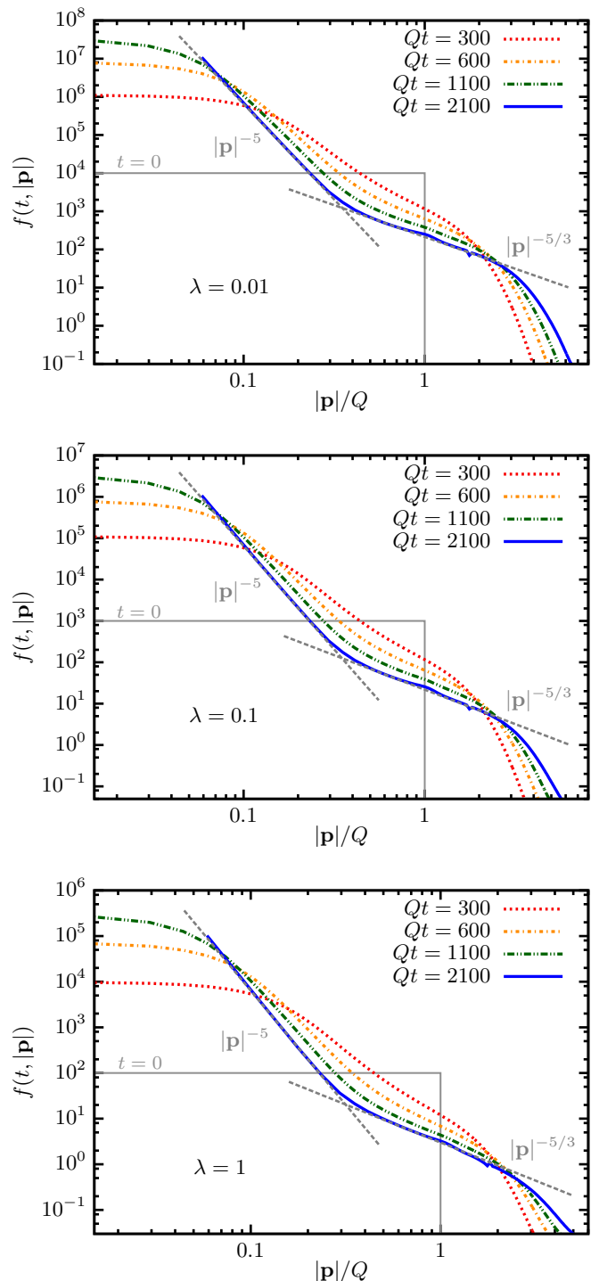
Figure 3. Particle number distribution for fluctuation initial conditions with \lambda = 0.01, 0.1, 1 (top to bottom) at different times including the initial time (gray). The approximate power laws with exponents \kappa_N = 5 and \kappa_E = 5/3 characterize the dual cascade in the respective momentum ranges (dashed gray lines).
