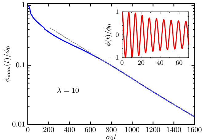
Figure 16. For \lambda = 10 , we observe an exponential decay of the field amplitude \phi_{\max}(t) with a rate of about \sim 10^{-3}\sigma_0 (dashed line).
