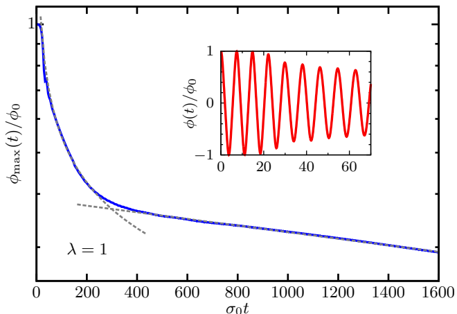
Figure 15. For \lambda = 1 , the power law of the field amplitude \phi_{\max}(t) is \sim t^{-c} with c \approx 0.4 for intermediate times (note the log-lin plot). At later times, an exponential damping with a small rate \sim 10^{-4}\sigma_0 is found.
