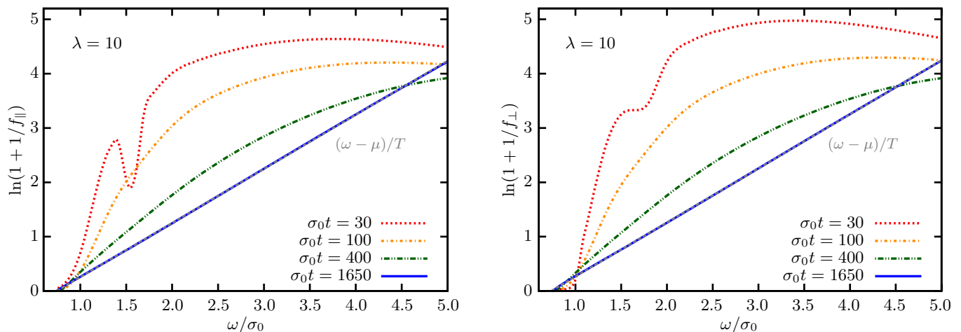
Figure 12. Longitudinal ( \parallel , left ) and transverse ( \perp , right ) inverse slope parameters \ln(1 + 1/f_{\parallel,\perp}) for macroscopic field initial conditions with \lambda = 10 at different times. We observe the approach to thermal equilibrium. For comparison, the dashed line in each plot corresponds to a Bose-Einstein distribution with temperature T \approx \sigma_0 and chemical potential \mu \approx 0.7\sigma_0 .
