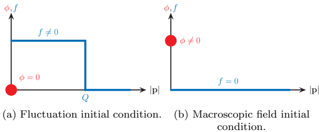
Figure 2. Illustration of the employed initial condition scenarios.
