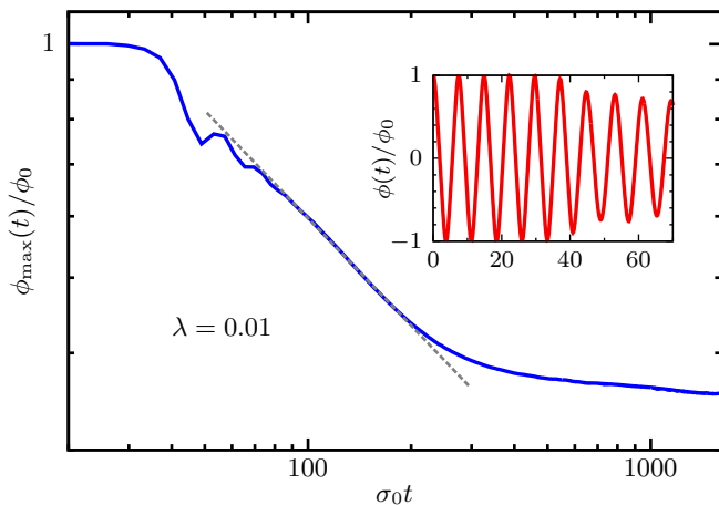
Figure 14. Double-logarithmic plot of the time evolution of the envelope \phi_{\max}(t) normalized to its initial value \phi_0 for \lambda = 0.01 . In the inset, the oscillating field is displayed. The field amplitude is \sim t^{-c} with c \approx 0.5 at intermediate times and with a much smaller exponent of the order of a few percent during the turbulent stages of the evolution at later times.
