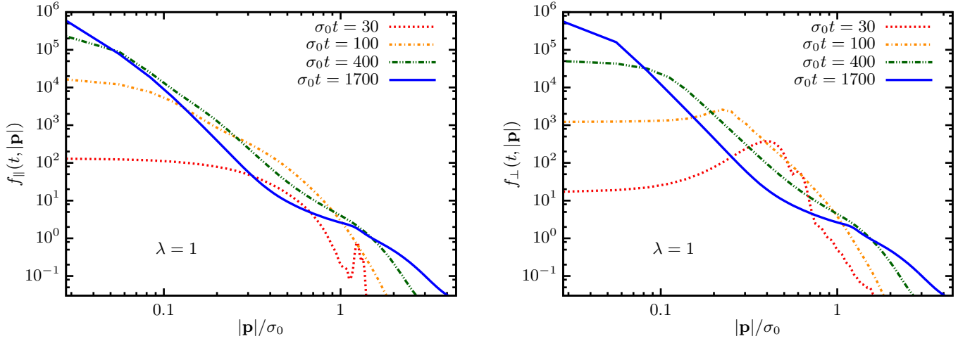
Figure 10. As in Fig. 9, but for \lambda = 1 , for which the system is still showing a dual cascade picture.
