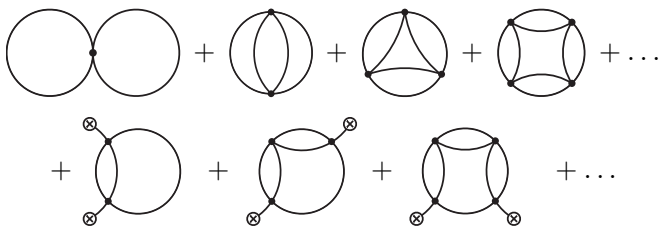
Figure 1. Diagrammatic representation of the infinite series of contributions to the free energy density at NLO in the 1/N expansion of the 2PI effective action. The lines denote self-consistent propagators, solid circles denote vertices and crosses denote field expectation values.
