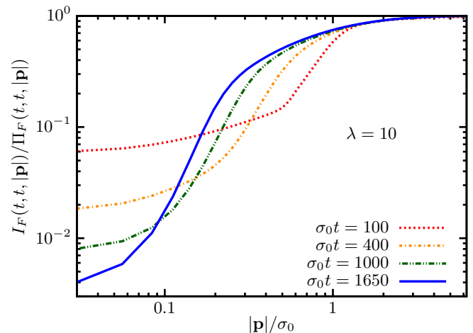
Figure 17. The ratio (24) for macroscopic field initial conditions with \lambda = 10 for different times.
