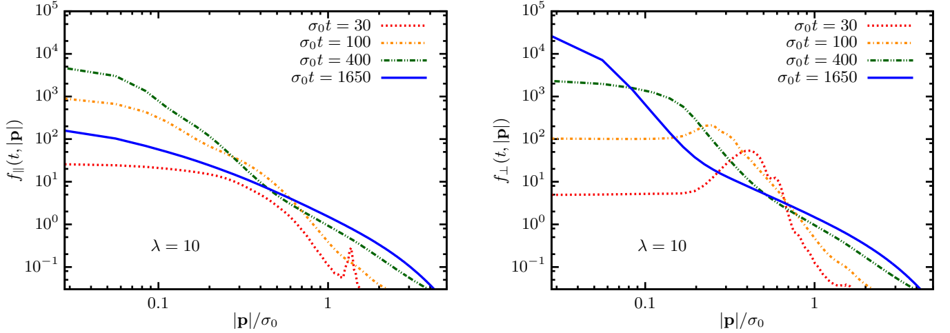
Figure 11. As in Fig. 9, but for \lambda = 10 , where strong deviations from the dual cascade picture occur. The longitudinal spectrum approaches thermal equilibrium rather quickly. At the same time, the transverse occupation number distribution exhibits a cascade-like behavior for small momenta, while the ultraviolet already shows signs of thermalization.
