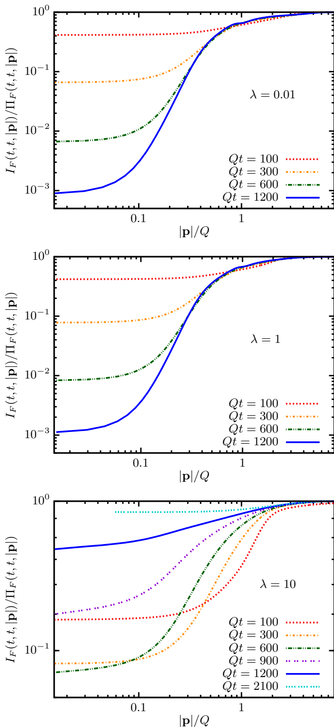
Figure 7. The ratio (24) for fluctuation initial conditions with \lambda = 0.01, 1, 10 (top to bottom). In a perturbative regime, I_F is expected to be dominated by the lowest one-loop contribution \Pi_F such that the ratio (24) is about one. While at high momenta the ratio approaches unity, in the infrared regime one observes very strong deviations from one for times where the transient inverse particle cascade occurs.
