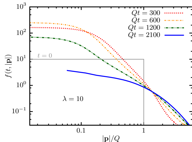
(a) Particle number distribution.
