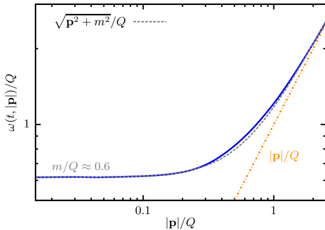
Figure 4. Dispersion relation for fluctuation initial conditions with \lambda = 0.01 at Qt = 1200 exhibiting an effective mass gap m . A fit to the quasiparticle dispersion relation \sqrt{\mathbf{p}^2 + m^2} is performed in good agreement with the numerical data for m/Q \approx 0.6 . Additionally, a linear dispersion relation, \omega = |\mathbf{p}| , is shown for comparison.
