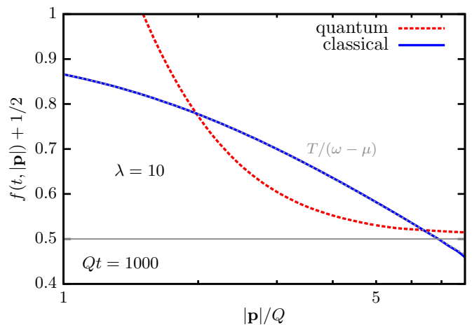
Figure 8. The sum f(t, |\mathbf{p}|) + 1/2 for \lambda = 10 at time Qt = 1000 for the quantum (dashed line) and the classical (solid line) evolution for fluctuation initial conditions. In addition, we show the classical thermal function T/(\omega(\mathbf{p}) - \mu) (gray, dotted) for comparison, with parameters as described in the main text. One observes that, in contrast to the quantum evolution, the classical results for f(t, |\mathbf{p}|) + 1/2 drop below 1/2 at high momenta, showing the decay of the initial quantum-half.
