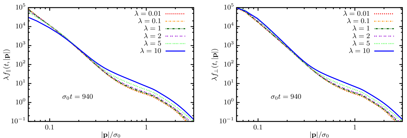
Figure 13. Rescaled longitudinal ( \parallel , left ) and transverse ( \perp , right ) occupation number distributions for macroscopic field initial conditions at fixed time \sigma_0 t = 940 for different values of the coupling \lambda .
