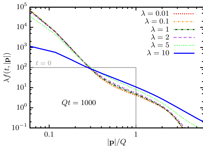
Figure 6. Rescaled particle number distribution for fluctuation initial conditions at fixed time for different values of the coupling \lambda . In the range \lambda \lesssim 2 , one observes that all curves collapse onto a single curve to good accuracy. In contrast, for stronger couplings sizable deviations occur.
