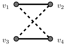
FIGURE 5. The switching encoded by the two directed edges \vec{S} = \{(v_1, v_2), (v_3, v_4)\} replaces the unoriented edges \{v_1, v_2\}, \{v_3, v_4\} by \{v_1, v_4\}, \{v_2, v_3\} .
