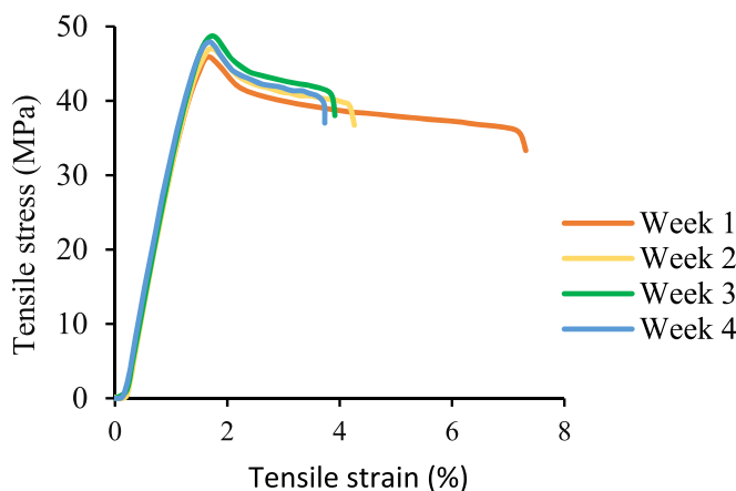
Figure 4. The tensile stress–strain curve for the degradation samples.
