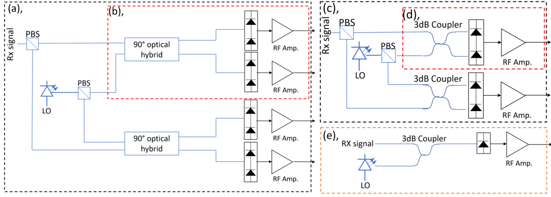
Fig. 1: Coherent receiver architectures. (a): Full coherent receiver (b): Single polarisation intradyne receiver (c): Polarisation diverse heterodyne receiver (d): Single polarisation heterodyne receiver (e): Minimal coherent receiver
