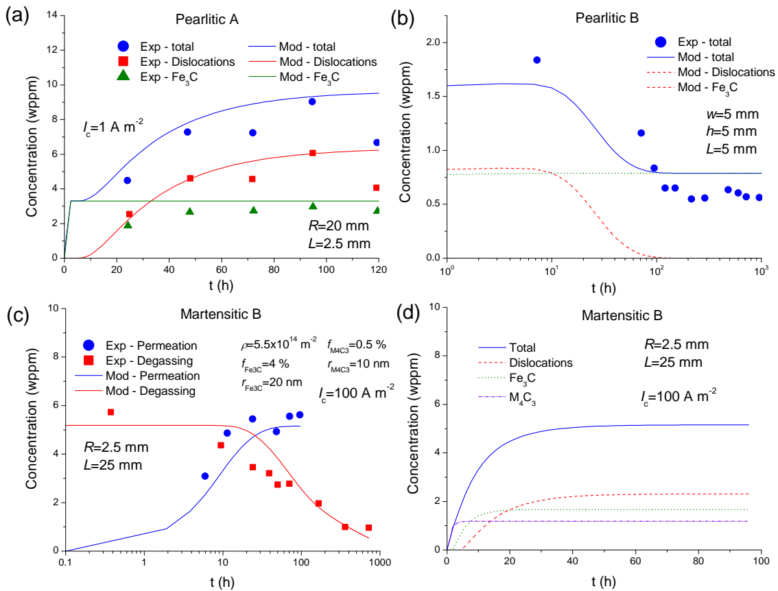
Figure 4: (a) Charging and (b) degassing profiles in pearlite. (c) Charging/degassing profiles in Martensitic B and (d) the relative contribution of various microstructural features to the total concentration.
