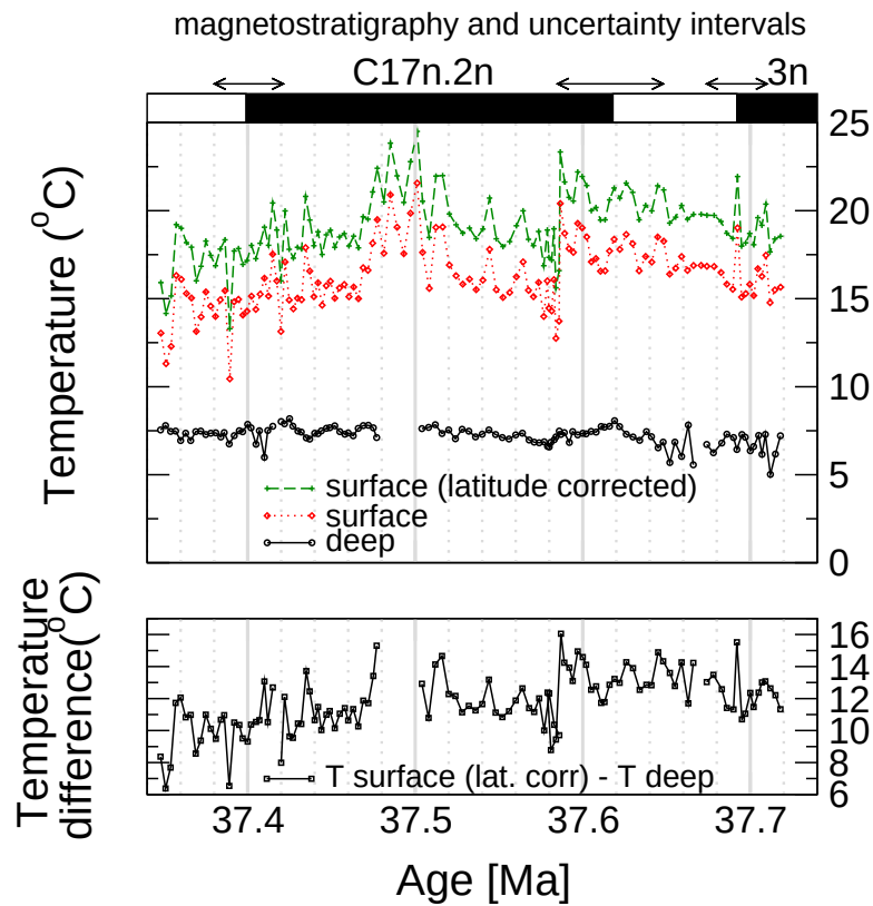
Figure 4.3: Temperature estimates from benthic and planktonic oxygen isotope data, using the assumption that variations in oxygen isotope values reflect changes in water temperature only (rather than salinity or ice volume). Benthic oxygen isotope values were species corrected for sea water disequilibrium effects (see text). Calculations were performed using the equation from Erez and Luz (1983) [182]. For the planktonic data, a second calculation was performed to correct for latitude dependent salinity variations in surface waters (Zachos et al. , 1994 [179]). The bottom panel shows the difference between latitude corrected surface water temperature and those estimated from the benthic record.
