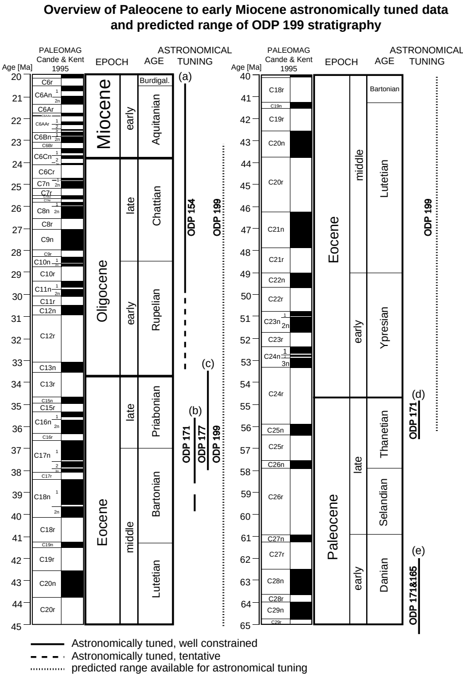
Figure 6.1: An overview of geological data that have been astronomically calibrated for parts of the Cenozoic. The dotted line shows the stratigraphic range predicted for the recovery of material during ODP Leg 199. The oldest age of sediment from Leg 199 is constrained by the estimated age of basement (~56-57 Ma). References to the calibrated sections are (a) [55; 155] (b) this study, and [135], (c) this study, (d) [161; 222], and (e) [103]. The time scale is that of Cande and Kent (1995) [46].
