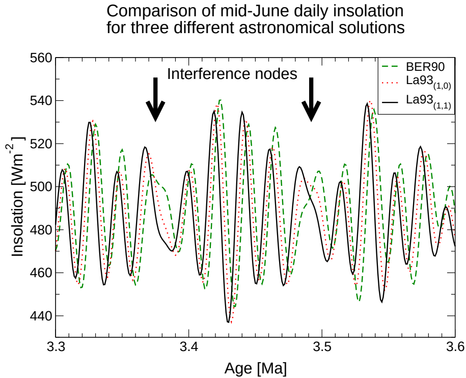
Figure 2.2: This plot shows three different astronomical calculations of mid-monthly June insolation at 65^\circ North. The calculation \text{La93}_{(1,0)} is that of Laskar (1990) [85]. The model BER90[80] uses the same eccentricity calculation but is based on a different calculation for obliquity and climatic precession. \text{La93}_{(1,1)} [86] is similar to \text{La93}_{(1,0)} , but includes a tidal dissipation term for the Earth-Moon system. Arrows indicate the position of “nodes” that result from interference between the obliquity and climatic precession components. This leads to a relative change in amplitude for the two closest peaks, and can affect the interpretation of individual cycles in the geological record. This problem can be addressed by considering the longer term amplitude modulation patterns.
