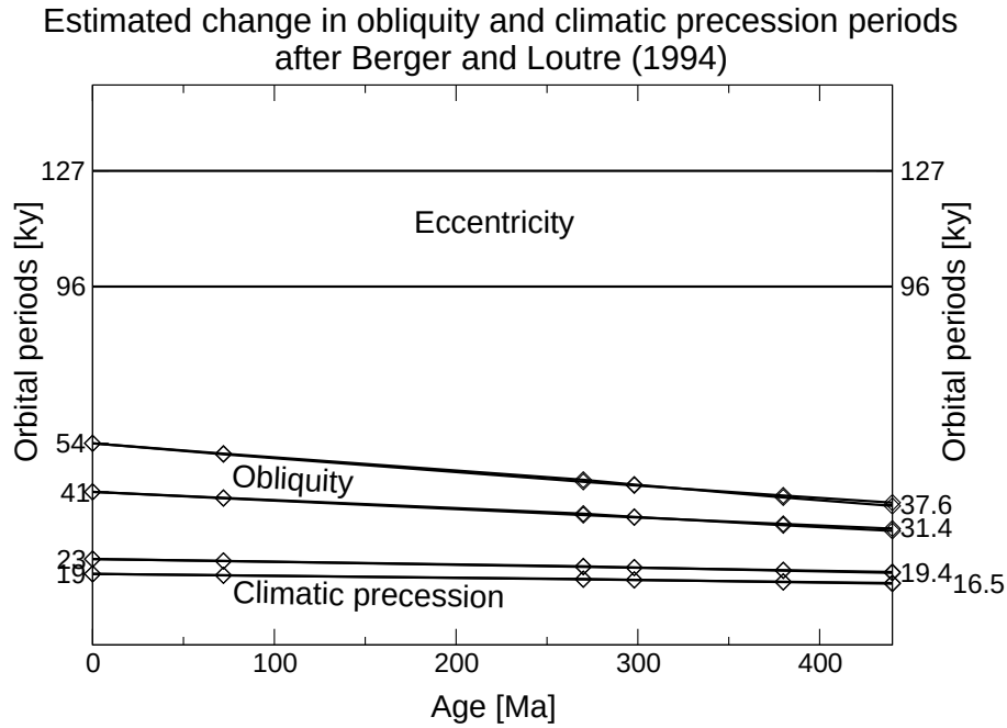
Figure 1.6: Estimated changes in the obliquity and climatic precession periods related to a changing Earth-Moon distance over the last 440 My, according to Berger et al. (1989) [95], and Berger and Loutre (1994) [96]. Note that the periods of obliquity and climatic precession change due to a change of the precession constant p , while the eccentricity periods remain unaffected. Note that this figure is for illustrative purposes only, as the exact variation of orbital frequencies over tens of millions of years is not yet known in detail.
