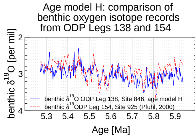
Figure 2.30: Comparison of benthic oxygen isotope data from ODP Leg 138 (Site 846, age model H) and ODP Leg 154, Site 925 after Pfuhr (2000) [130].
