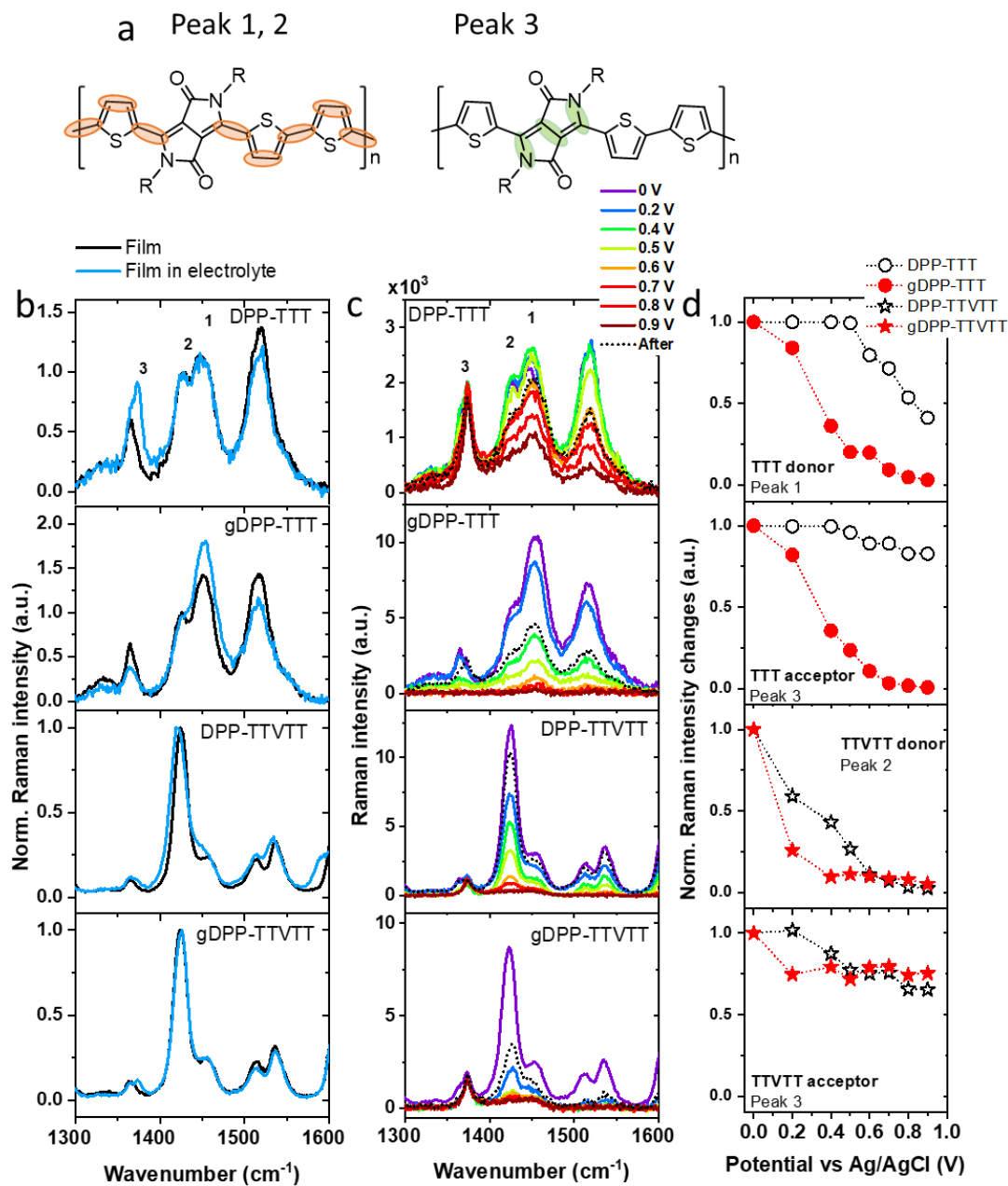
Figure 4. (a) Raman peak assignments of the main 3 vibrational mode labelled on the spectra, which correspond to mainly donor (peaks 1 and 2) and acceptor units (peak 3). (b) Raman spectra of the 4 copolymers thin films in air and immersed in acetonitrile electrolyte with TBAPF 6 , using 488 nm excitation wavelength. (c) In-situ electrochemical Raman measurements using 488 nm excitation wavelength during chronoamperometric applied potentials at constant 0 to 0.9 V oxidizing bias. (d) Normalized Raman intensity changes for peaks 1 – 3 extracted from the in-situ electrochemical Raman spectra.
