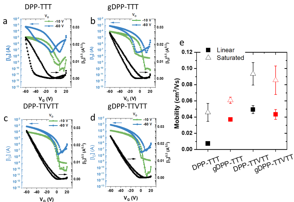
Figure 2. a-d) OFET transfer plots ( I_D - V_G and I_D^{0.5} - V_G ) for a set of 5 \mu\text{m} channel length, sweeping V_G from 20 to -60V and constant V_D = -10 and -60 V. (e) OFET linear and saturated hole mobility values extracted using an average of transfer characteristics. Error bars indicate the standard deviation extracted from a collection of 4 device channels per copolymer.
