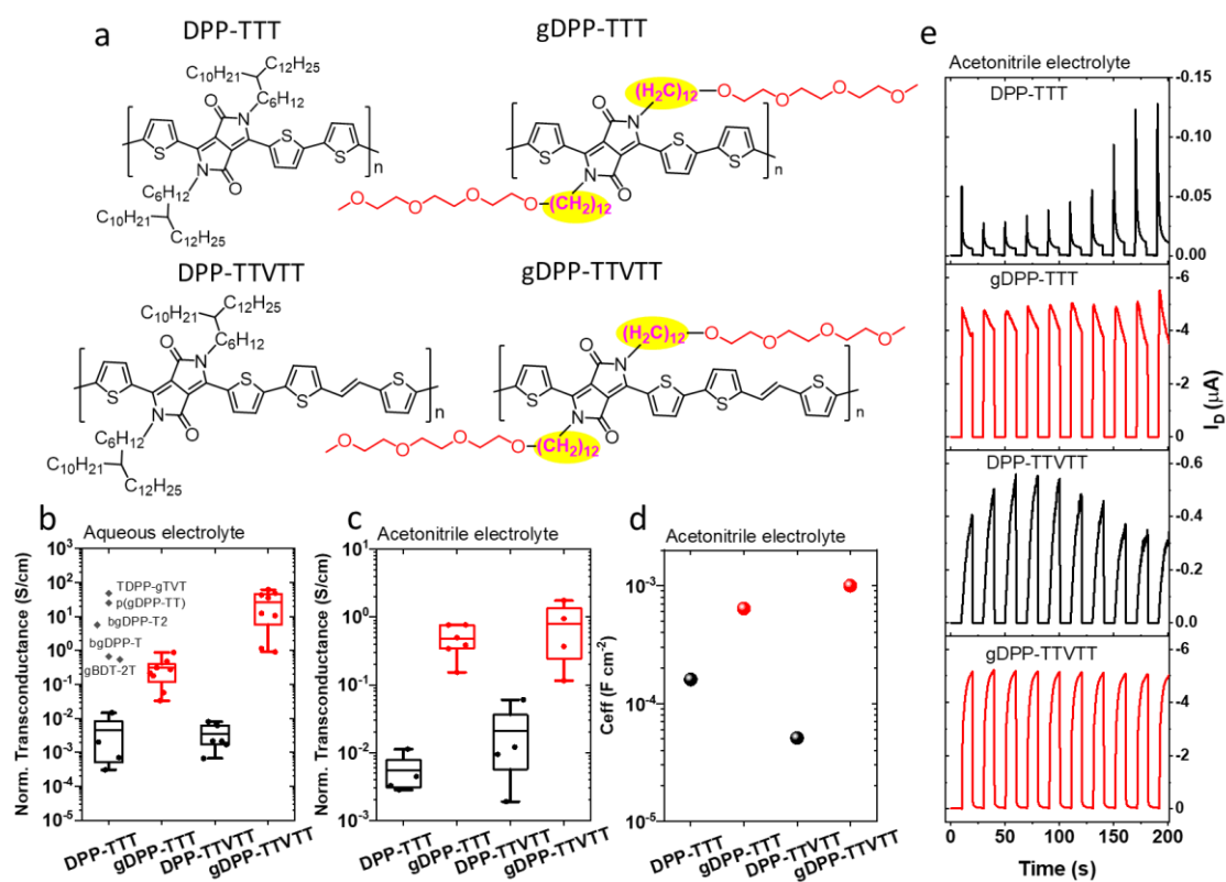
Figure 1. (a) Chemical structures of the 4 DPP copolymers: DPP-TTT, gDPP-TTT, DPP-TTVTT and gDPP-TTVTT. OECT maximum transconductances normalized by Wd/L of multiple devices using (b) ringer's solution (2mm/200 \mu\text{m} – W/L) and (c) 0.1M TBAPF 6 acetonitrile electrolyte (100/10 \mu\text{m} - W/L), taken from the derivative of the transfer characteristics. Each datapoint represents a device and the additional values marked as grey diamonds in (b) are taken from literature for comparison with other similar copolymers. [26–28,34] The statistical box plot with individual device data points show the device-to-device variation including a mean line, box data range of 25 and 75% and whiskers of max and min values. (d) The effective capacitance per unit area at 1Hz extracted using a modified Randles cell equivalent circuit R_s(Q_p||R_p) shown in SI. (e) Transient OECT measurement of drain current changes over 200 s while the gate bias is pulsed between 0 and -0.8 V for OFF and ON regimes, respectively.
