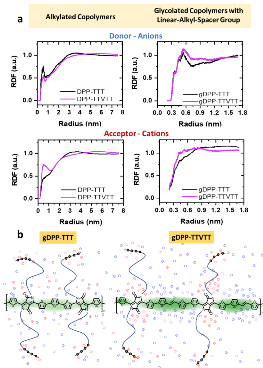
Figure 5. a) The graphs show the radial distribution functions (RDF) of cations and anions from the conjugated backbone, calculated from MD simulations in acetonitrile with TBAPF 6 . The donor-anion and acceptor-cation RDFs are significantly higher at lower radius for glycolated copolymers (below 0.7 nm), indicating more ions localized closer to the backbone compared to the alkylated counterparts. b) A schematic representation of the cation (red) and anion (blue) distribution in the glycolated copolymers. This illustrates the density of ions, which is greater in gDPP-TTVTT than DPP-TTT due to the reduced sidechain attachment frequency. Therefore, gDPP-TTVTT could result in more readily formed polarons (green) localized to the donor units, where there are more mobile anions.
