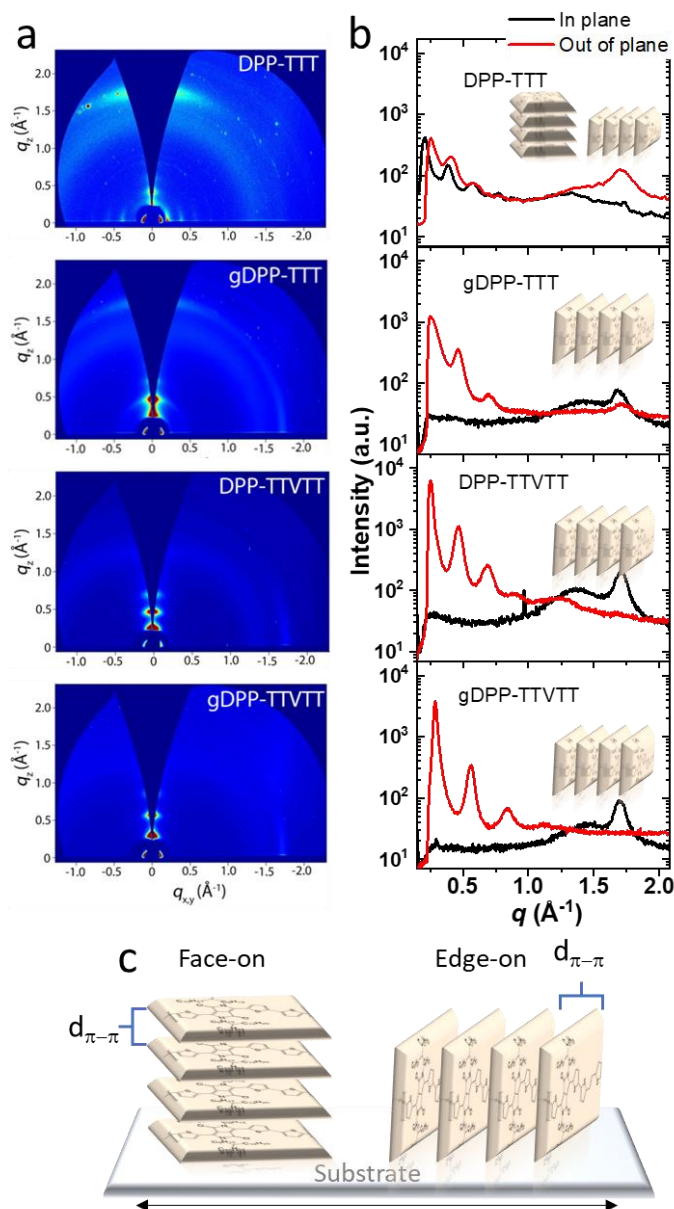
Figure 3. (a) 2D GIWAXS patterns for the 4 copolymers and (b) GIWAXS diffractograms for in-plane and out-of-plane scattering with illustrative insets of the dominant molecular orientation that the copolymer adopts in thin films. DPP-TTT has a ‘face-on’ dominant bimodal orientation whereas all other copolymers adopt ‘edge-on’ orientation. (c) Illustration of the structural packing orientations including ‘face-on’ and ‘edge-on’ relative to the substrate.
