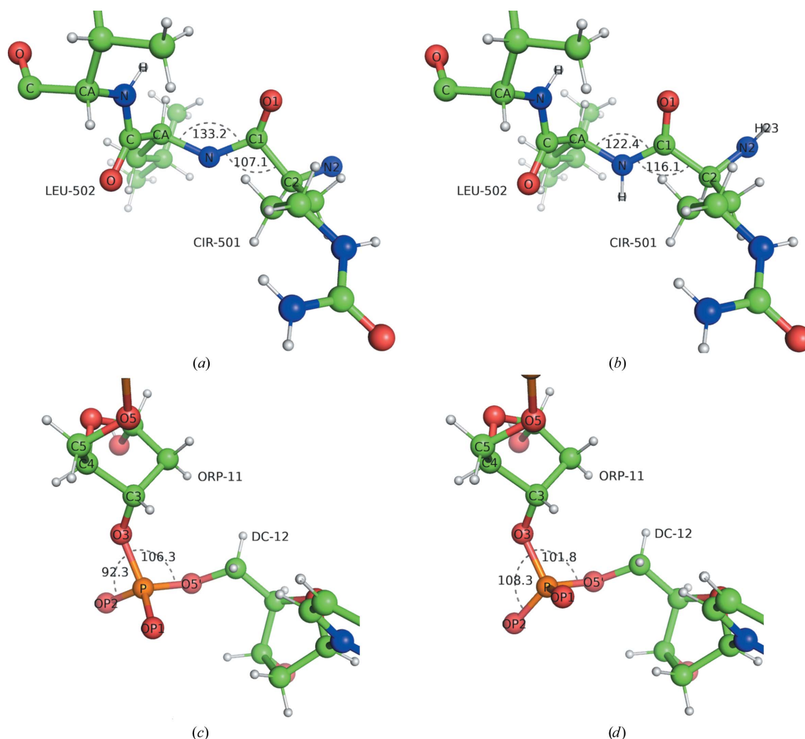
Figure 2 ( a, b ) PDB entry 1ol1 and ( c, d ) PDB entry 3waz after 20 cycles of geometry optimization using the Servalcat REFMAC5 controller ( a, c ) without and ( b, d ) with the alias mechanism. Since the monomers CIR ( a, b ) and ORP ( c, d ) do not follow the standard nomenclature, their chemistry is not properly recognized without the alias mechanism (missing hydrogen atoms in peptide bonds and missing restraints other than bond length). The ideal bond angles in the CCP4-ML are CA–C–N, 115.9°; C–N–CA, 122.1° (for a peptide link); O3'–P–OP2, 108.5°; O3'–P–O5', 101.1° (for a phosphodiester link). Images were created using PyMOL (version 2.4; Schrödinger).
