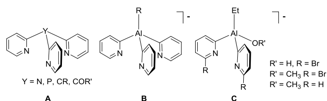
Scheme 1 (A) Frameworks found in the family of tris-2-pyridyl ligands, (B) anionic tris-2-pyridyl aluminate ligands, and (C) heteroleptic aluminium complexes.
