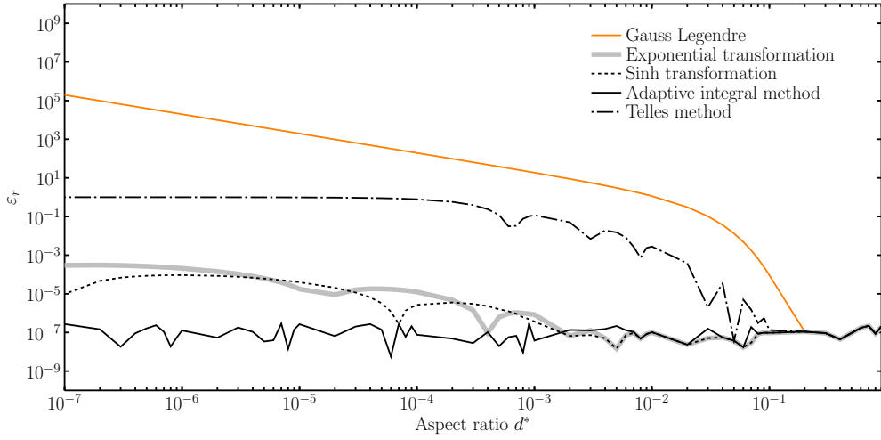
Figure 4: Relative errors obtained by different methods for strong nearly singular integral on line isogeometric element
