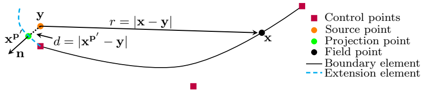
Figure 11: Minimum distance d to the extension element when \mathbf{x}^{p'} \notin \Gamma_e
