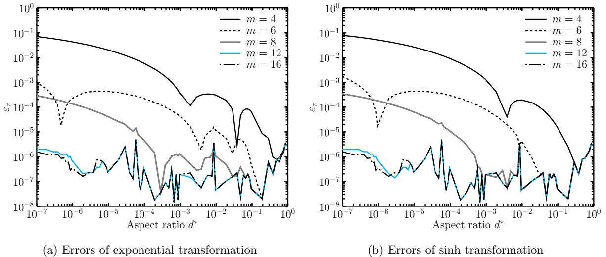
Figure 7: Errors of exponential and sinh transformations change when different numbers of Gauss points are used for the weak nearly singular integral
