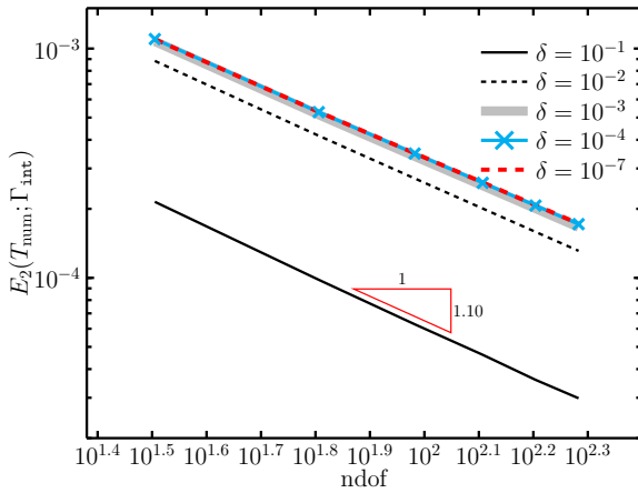
Figure 30: Solution convergence for different \delta
