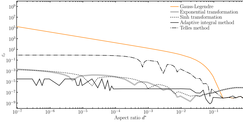
Figure 6: Relative errors obtained by different methods for strong nearly singular integral on arc isogeometric element
