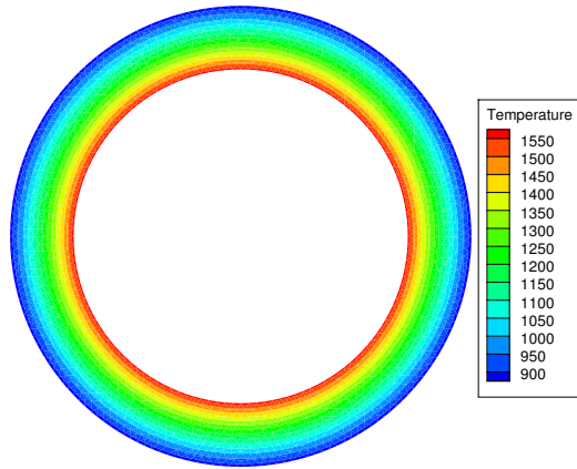
Figure 32: Temperature distribution with \delta = 10^{-6} m
