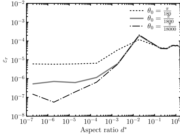
Figure 13: Relative errors obtained by extended sinh transformation for strong nearly singular integral on arc isogeometric element
