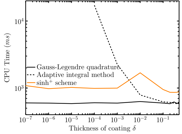
Figure 22: Comparisons of CPU time for different methods
