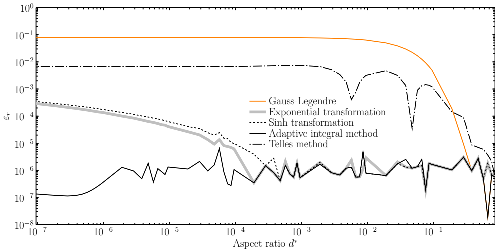
Figure 5: Relative errors obtained by different methods for weak nearly singular integral on arc isogeometric element
