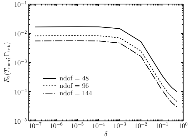
Figure 24: L_2 relative error norm E_2(T_{\text{num}}; \Gamma_{\text{int}}) vs. \delta
