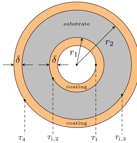
Figure 20: The thermal resistance network for heat transfer through a cylinder with multilayer coating structures
