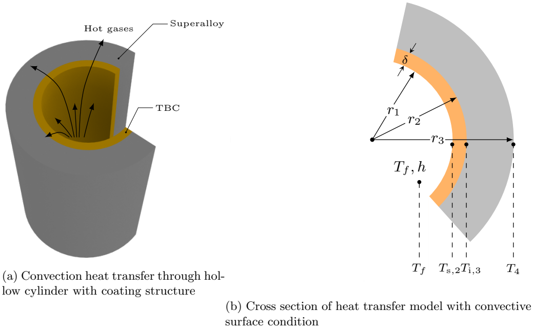
Figure 27: Convection heat transfer model
