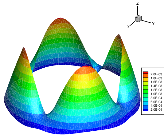
Figure 33: Relative error in the temperature
