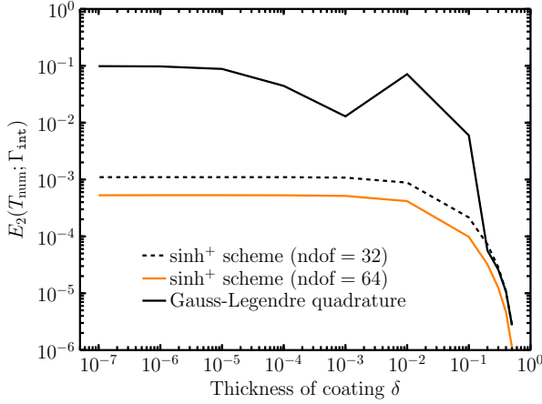
Figure 28: L_2 norm E_2(T_{\text{num}}; \Gamma_{\text{int}})
