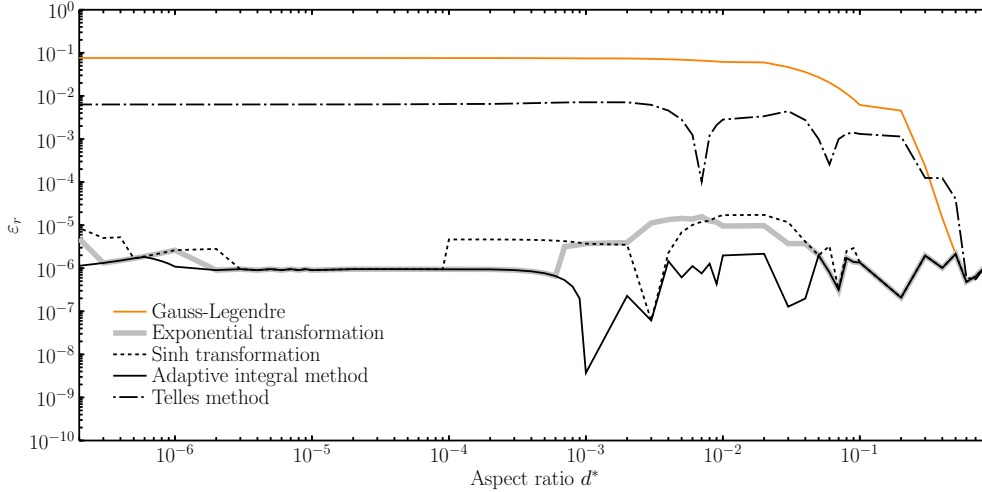
Figure 3: Relative errors obtained by different methods for weak nearly singular integral on line isogeometric element
