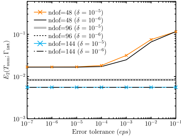
Figure 25: L_2 relative error norm E_2(T_{\text{num}}; \Gamma_{\text{int}}) when different error tolerances are used in \sinh^+ (illustrated in Figure 15)
