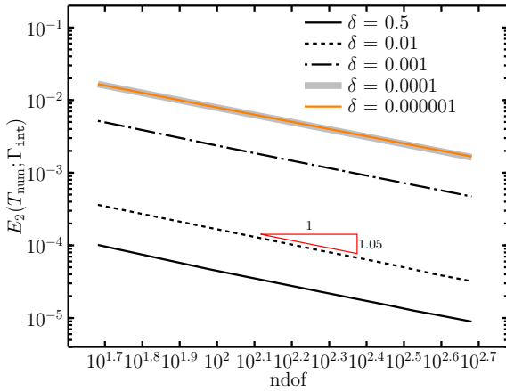
Figure 23: Convergence of L_2 relative error norm E_2(T_{\text{num}}; \Gamma_{\text{int}}) with ndof
