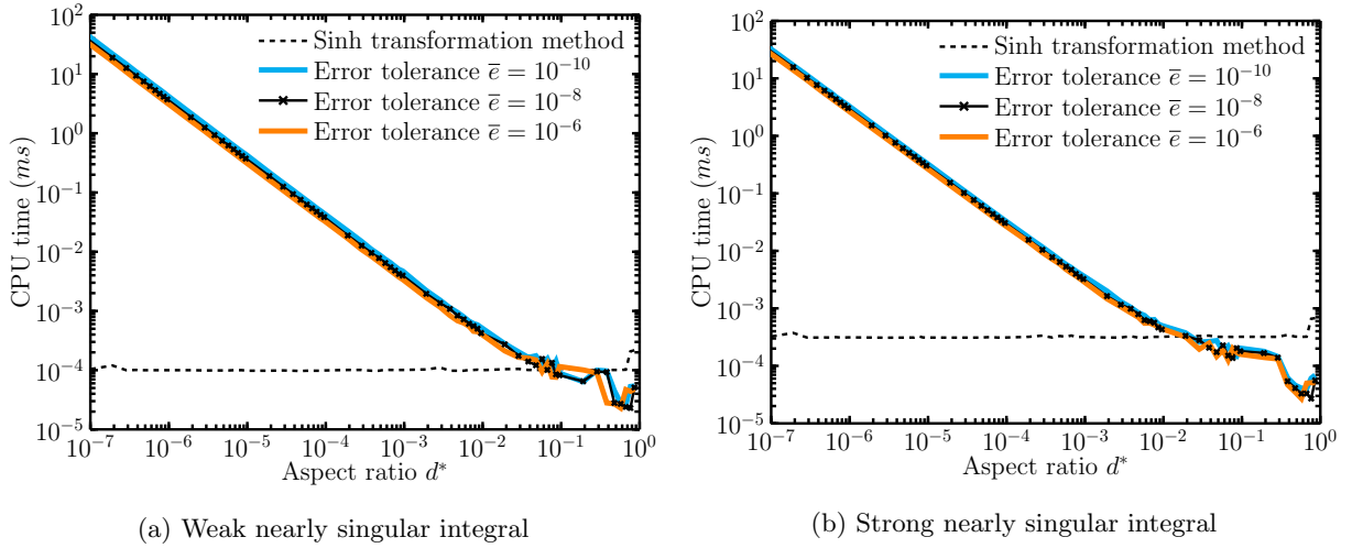
Figure 10: CPU time comparison between adaptive integral method and sinh transformation method on isogeometric arc element
