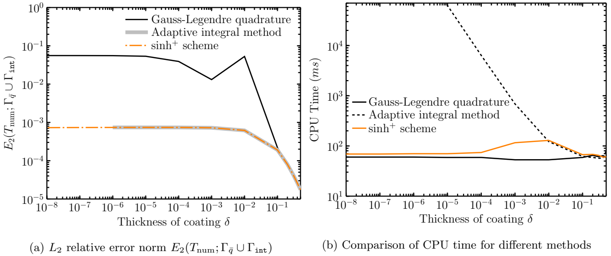
Figure 18: Comparisons of accuracy and efficiency
