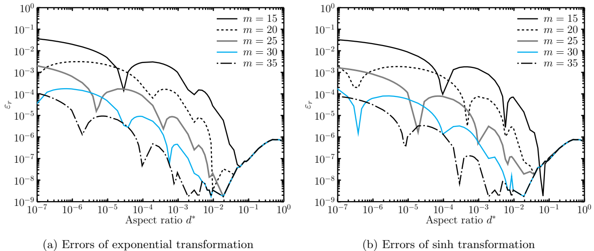
Figure 8: Errors of exponential and sinh transformations change when different numbers of Gauss points are used for the strong nearly singular integral
