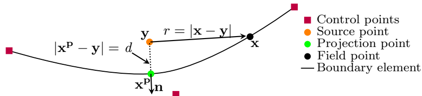
Figure 1: Minimum distance d to the element when \mathbf{x}^p \in \Gamma_e
