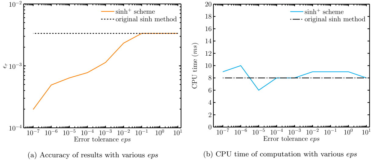
Figure 16: The impact of various \text{eps} on the accuracy and CPU time of the nearly singular integration
