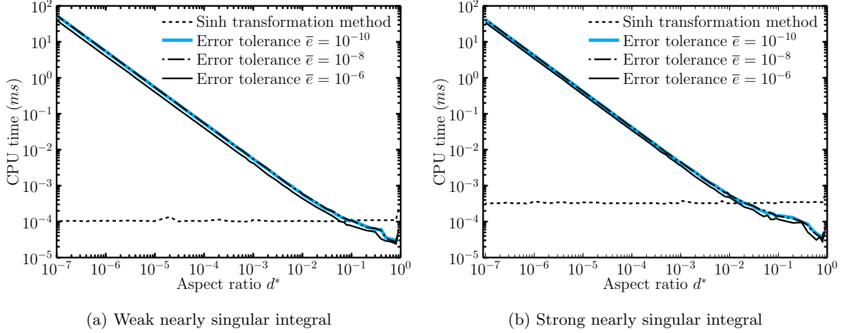
Figure 9: CPU time comparison between adaptive integral method and sinh transformation method on isogeometric line element
