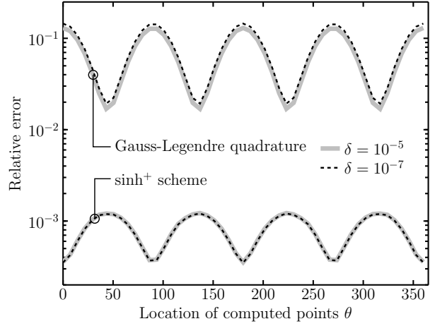
Figure 29: Relative errors along S_1 with \delta = 10^{-5} and 10^{-7}
