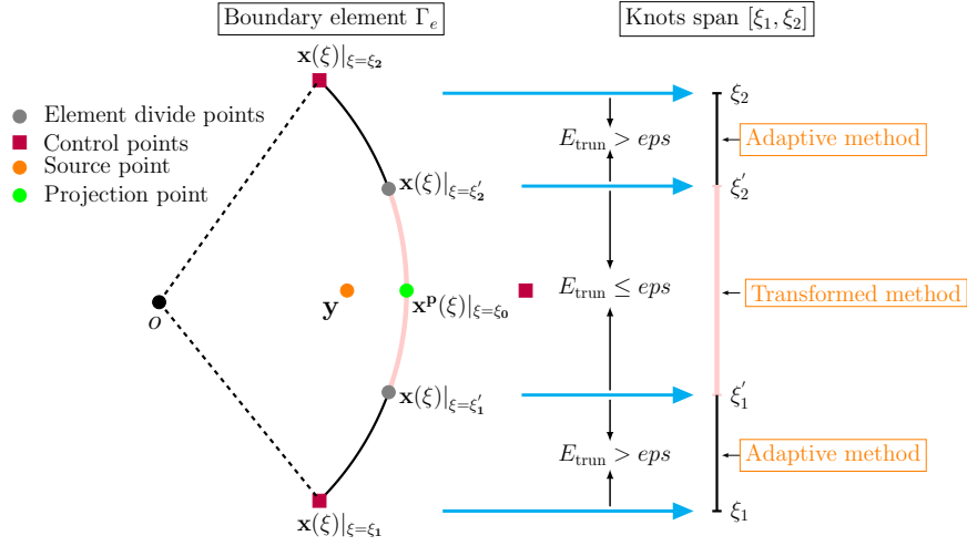
Figure 15: Choice of integral method based on the truncation errors E_{\text{trun}} of Taylor expansion
