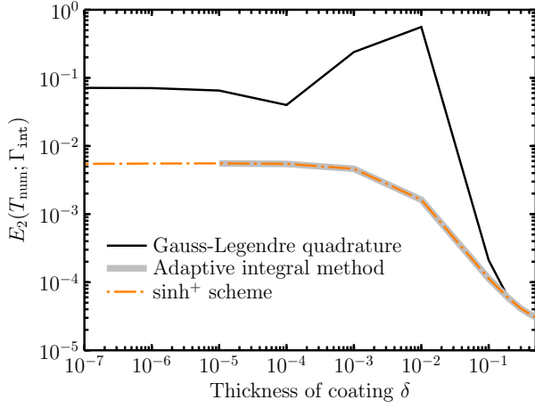
Figure 21: L_2 relative error norm E_2(T_{\text{num}}; \Gamma_{\text{int}})
