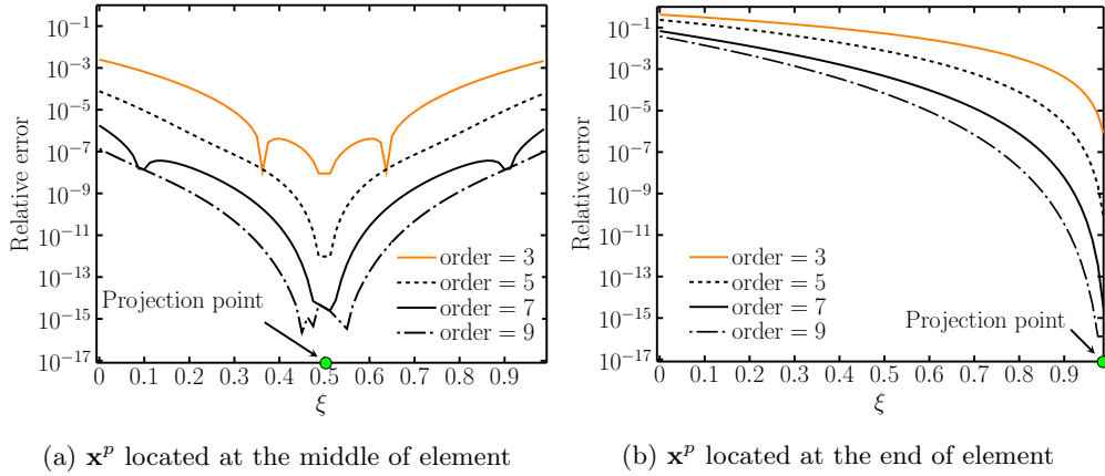
Figure 14: Comparisons of relative errors for different orders of Taylor expansion
