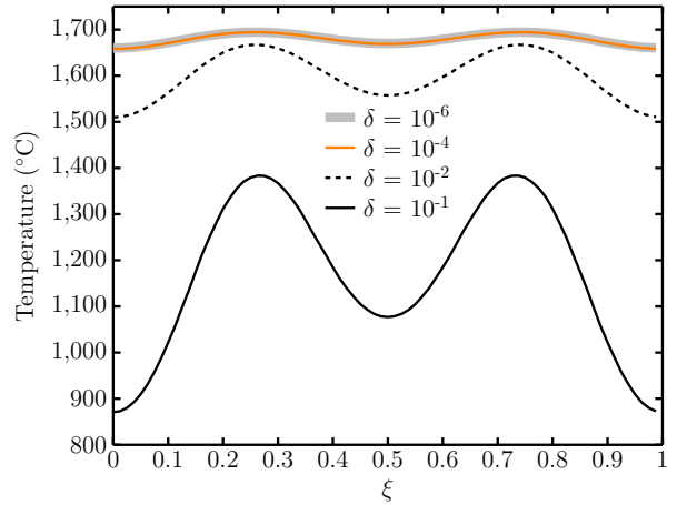
Figure 36: Interface temperature distributions
