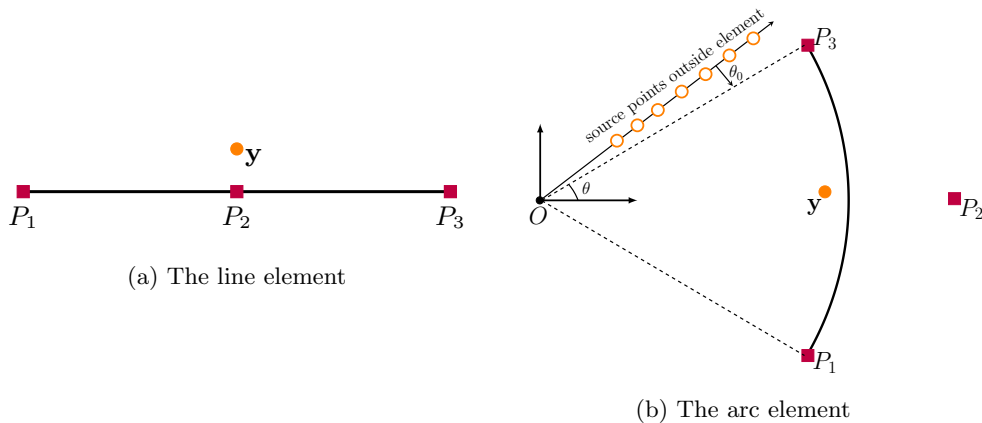
Figure 2: Considered isogeometric elements
