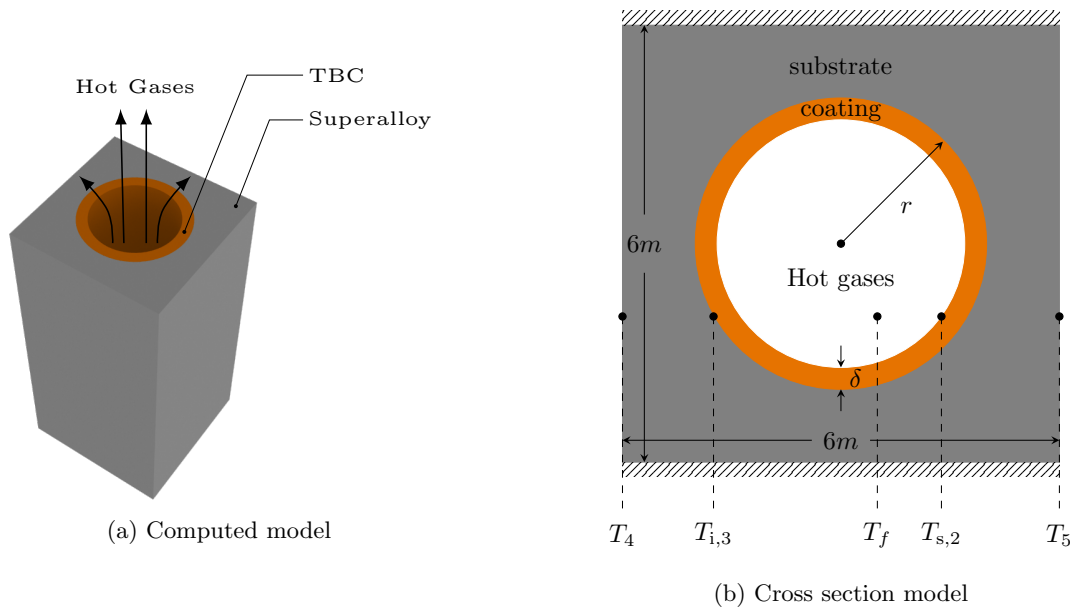
Figure 34: Convection heat transfer model
