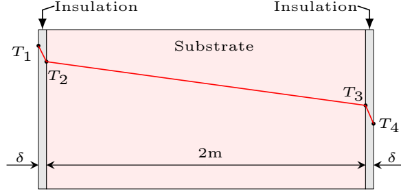
Figure 17: Heat transfer through a model with double flat coatings
