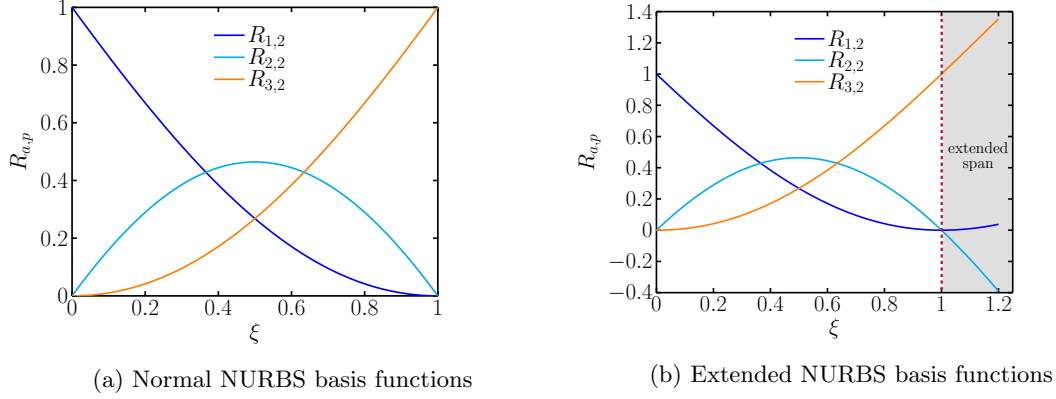
Figure 12: NURBS basis functions of the considered isogeometric element
