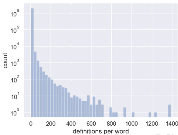
Figure 3: Number of definitions per term defined on Urban Dictionary (log scale) [22].
