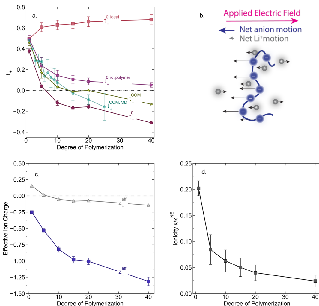
Fig. 4 (a) Transference number vs. degree of polymerization calculated using ideal solution conditions ( t_{+}^{\text{id,ideal}} ), ideal polymer conditions ( t_{+}^{\text{id,polymer}} ), and rigorous real solution conditions ( t_{+}^0 , t_{+}^{\text{COM}} ). t_{+}^{\text{id,ideal}} and t_{+}^{\text{id,polymer}} were calculated from PFG NMR measurements, while t_{+}^0 and t_{+}^{\text{COM}} were calculated from eNMR measurements. t_{+}^{\text{COM}} is reported to allow comparison with t_{+}^{\text{COM,MD}} that was calculated from course-grained molecular dynamic simulations reproduced from ref. 11. (b) Schematic of conditions leading to a negative transference number. (c) Effective ion charge for the anion and cation. (d) Ionicity ( \kappa/\kappa^{\text{NE}} ) vs. degree of polymerization. All experimental data corresponds to 0.5 m Li + whereas MD simulation data presented here corresponds roughly to a cation concentration of 0.48 M.
