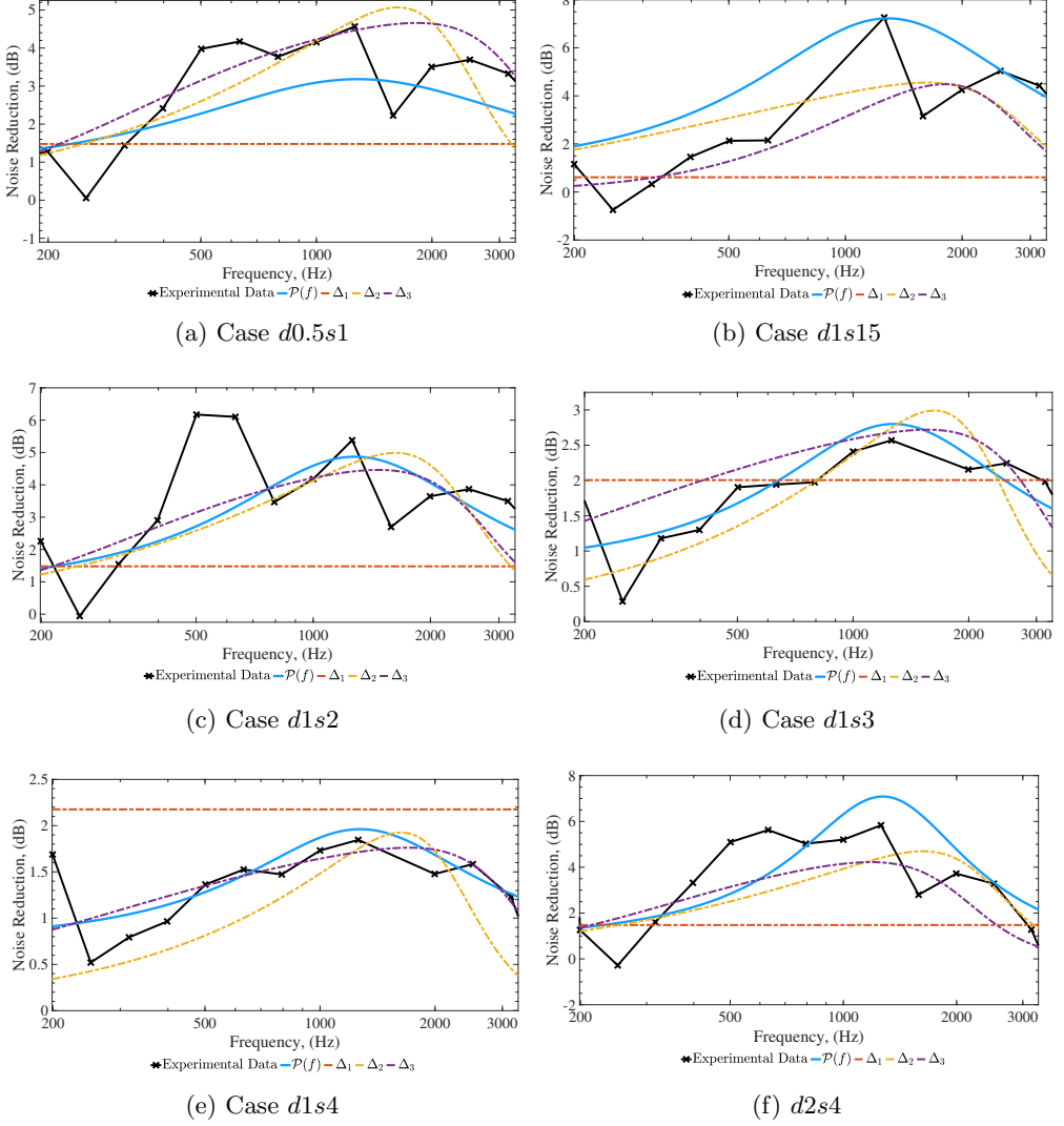
Figure 20: Comparison of predicted leading edge noise for the model \mathcal{P}(f) from (5.1) alongside experimental data taken from Geyer & Enghardt (2024) and models \Delta_{1,2,3} from (5.9).
