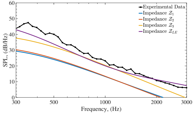
(c) Case 40 Porosity.
