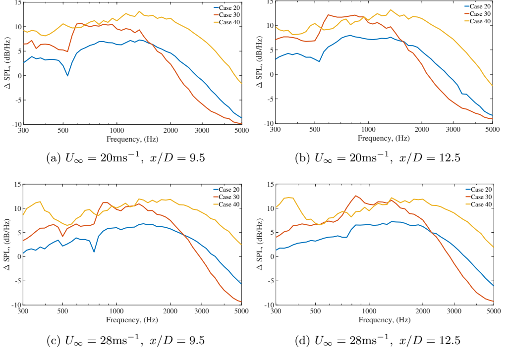
Figure 13: Noise reduction ( \Delta \text{SPL} ) for each flow condition when comparing the SPL from the rigid insert to each of the three porous insert cases tested.
