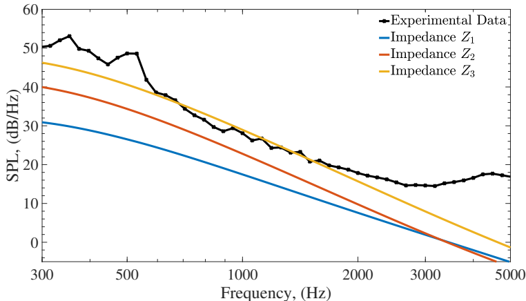
Figure 16: Comparisons of predicted leading edge noise for the U_\infty = 20\text{ms}^{-1} , x/D = 9.5 flow condition and the case 20 porous insert. We test impedance models Z_{1,2,3}(\omega) against the experimental data.
