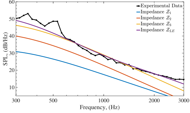
(a) Case 20 Porosity.
