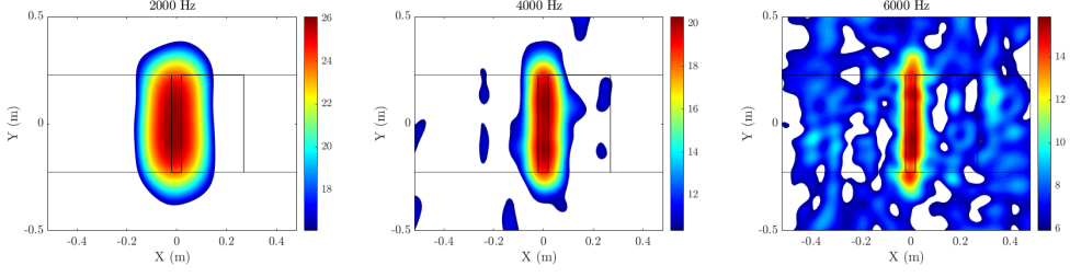
Figure 9: Beamforming maps for the Case 20 porous insert at three frequencies and mean flow velocity of 28\text{ms}^{-1} . The cylinder is 12.5D upstream of the leading edge. The flow is from left to right and the colorbar scale is given in dB.
