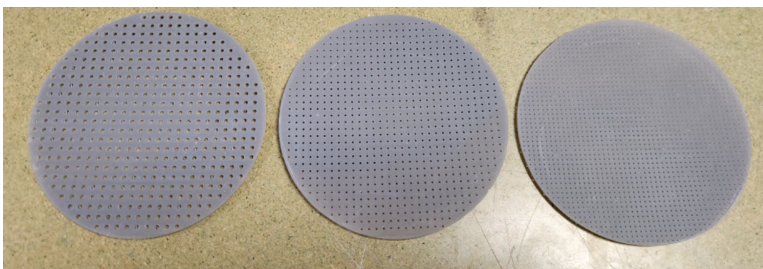
Figure 7: 3D printed samples of the three porosities investigated in this experiment. Left: Case 30, Middle: Case 20. Right: Case 40. Case 40 has the finest porous structure, but has the smallest distance between pores. Thus, it has the largest open area ratio due to the large number of pores per unit area.
