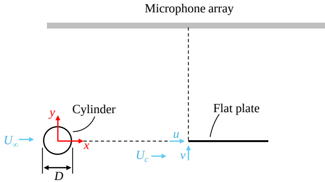
Figure 8: Schematic for the acoustics measurements of leading-edge noise in anisotropic turbulence. The leading-edge insert can be replaced with porous inserts as shown in Figure 2 of (Ayton et al. (2021b)).
