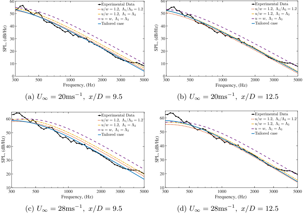
Figure 14: Comparison of predicted leading edge noise when varying streamwise to spanwise ratios within the turbulence model. Each flow condition is tested and only the rigid model is used.
