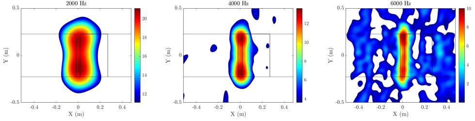
Figure 10: Beamforming maps for the Case 40 porous insert at three frequencies and mean flow velocity of 28\text{ms}^{-1} . The cylinder is 12.5D upstream of the leading edge. The flow is from left to right and the colorbar scale is given in dB.
