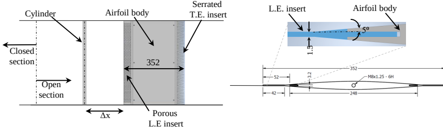
Figure 5: Schematic of the flat plate airfoil test model. Figure adapted and used with the authors' permission from (Ayton et al. (2021b)).
