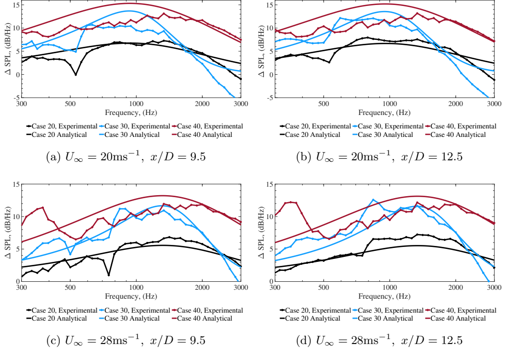
Figure 19: Predicted noise reduction using our leading-edge noise model that includes the full three-dimensional turbulence spectra and the impedance model Z_{LE}(\omega) , each porous insert case and flow condition are tested.
