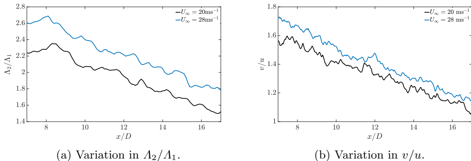
Figure 6: Variation of length scale and RMS velocity ratios with distance x/D from the cylinder.
