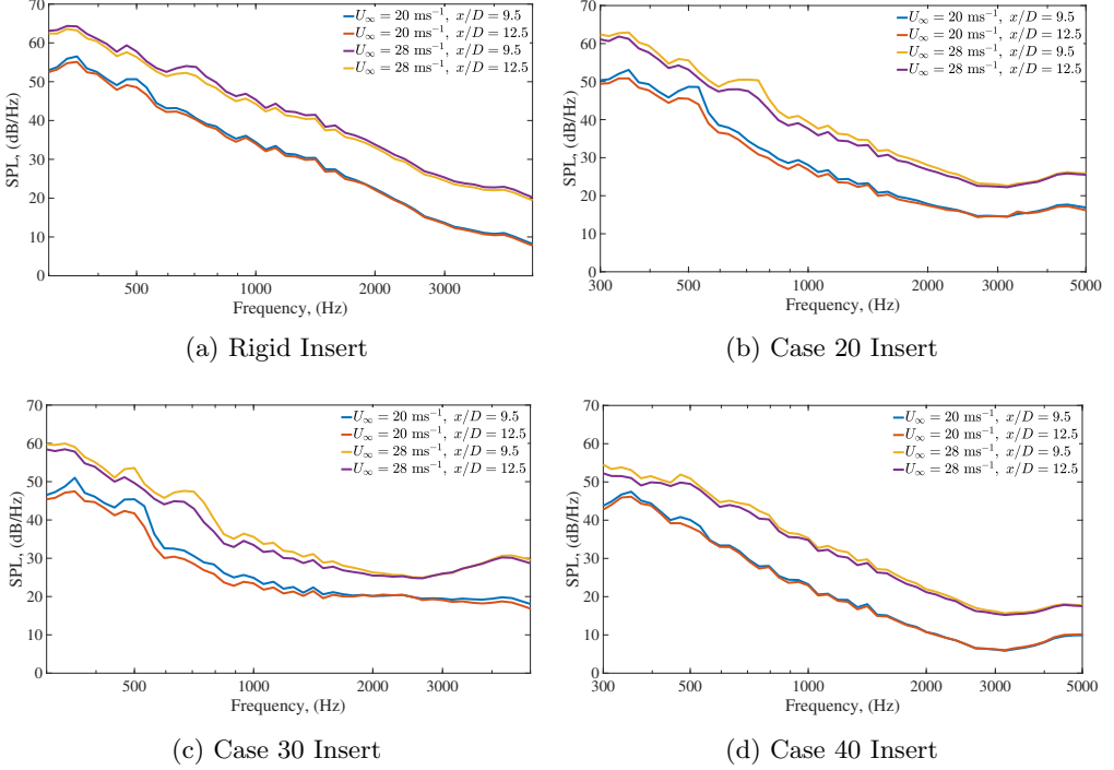
Figure 12: Comparisons for all tested leading-edge inserts as flow conditions (inflow velocity and cylinder distance) are changed.
