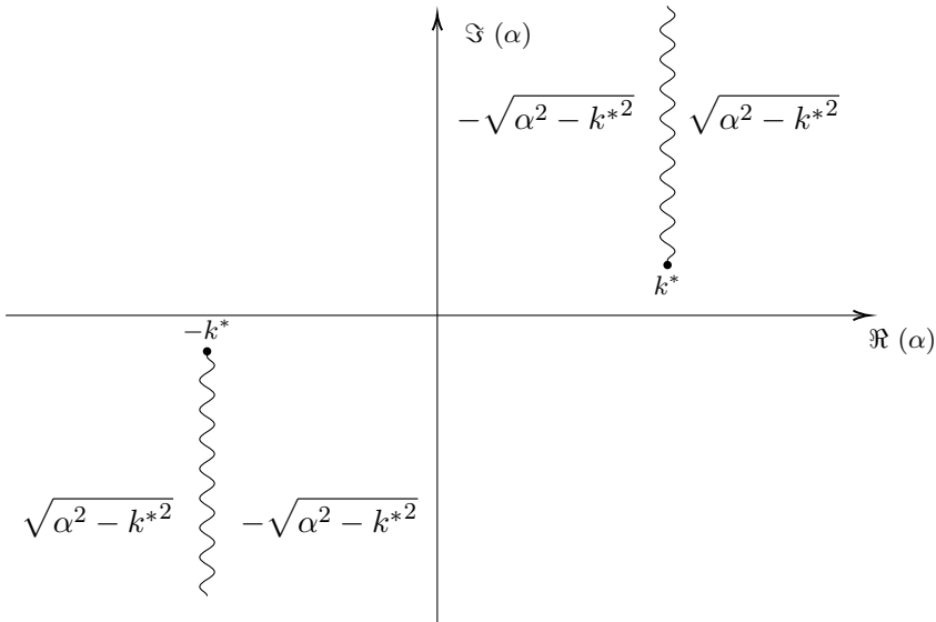
Figure 3: Demonstration of branch cuts \Gamma^{k,-k} and the values \gamma(\alpha) takes on each side. We take the square root in the diagram as the principle square root.
