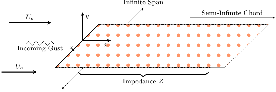
Figure 2: Mathematical setup for an incident gust scattering off of a semi-infinite porous plate.
