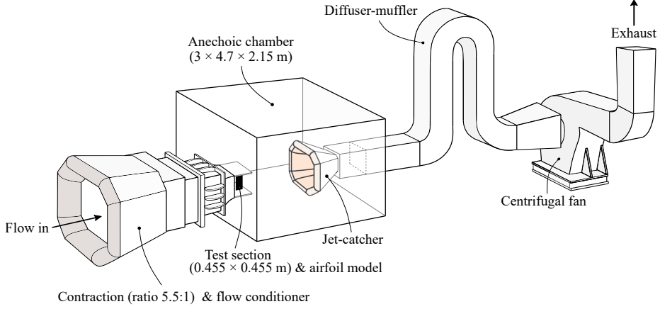
Figure 4: Schematic of UNSW anechoic wind tunnel.
