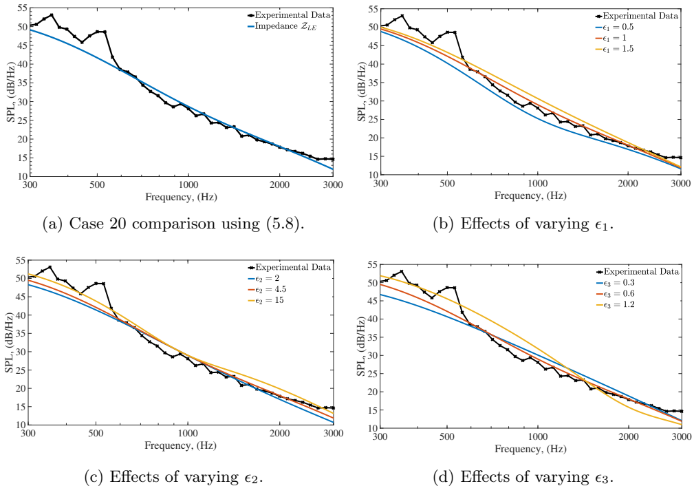
Figure 17: Changing Z_{LE}(\omega) to approximate the noise using Case 20 at U_\infty = 20 \text{ ms}^{-1} , x/D = 9.5 .
