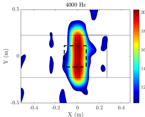
Figure 11: Region of integration for beamforming to obtain the frequency spectrum of the leading-edge SPL. The flow is from left to right and the colorbar scale is given in dB.
