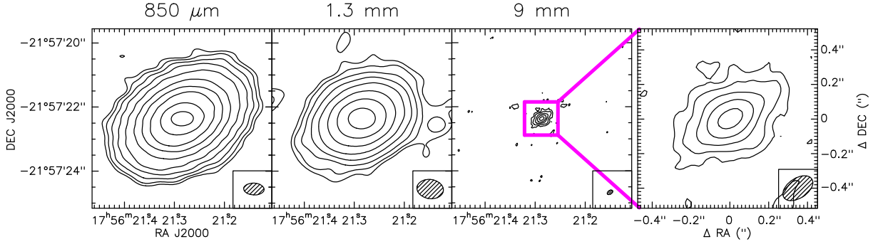
Fig. 1. Continuum maps at different wavelengths, from the left: 850 \mu\text{m} , 1.3 mm and 9 mm, this latter obtained from the combination of VLA 8.0 mm and 9.8 mm bands. The contour levels correspond to -3 (dashed), 3, 6, 12, 24, 48, 100, 200, 400, 800, 1600 \sigma . The bottom right of every panel shows the synthesized beam (see Table 1).
