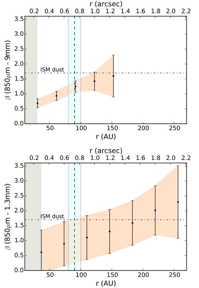
Fig. 11. Dust opacity power law index ( \beta ) profiles derived using Eq. 4. \beta(r) is computed between 850\mu\text{m} and 9 mm in the top panel and between 850\mu\text{m} and 1.3 mm in the bottom panel. The uncertainties are propagated from the surface brightness profiles presented in Fig. 9. The derived values of \beta(r) in the top panel are dominated by the low signal to noise in the VLA image from \sim 100 AU and are very uncertain beyond this radius. The CO snowline at 90 \pm 10 AU from Qi et al. (2015) is pictured as the dashed vertical line.
