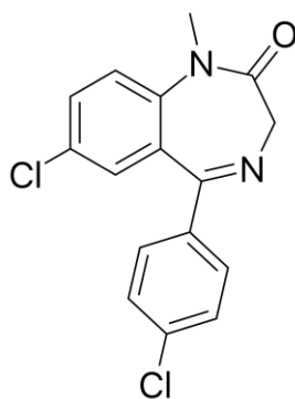
4-chloro-diazepam (Ro 5 4864)
