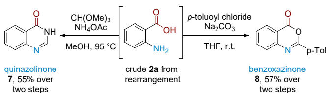
Scheme 2. Synthetic applications.
