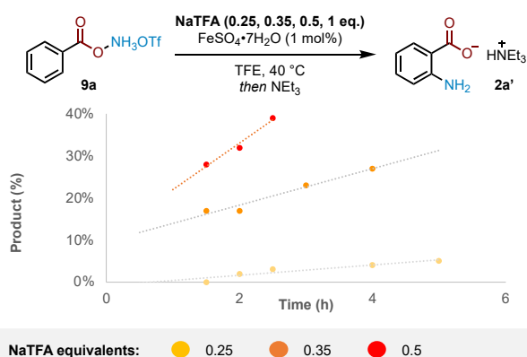
Figure 2. a) Reaction order analysis in NaTFA for triflate salt 9a . b) Rate-determining step (RDS) inference from rate of product formation with varying arene electronics. Yields determined by 1 H NMR using 1,2-DME as an internal standard after quenching with Et 3 N and filtering through silica
