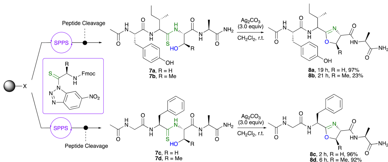
Scheme 3 SPPS on amide resin using Fmoc-amino acids and benzotriazolides to afford the requisite thioamide starting materials, 7 , after cleavage. These were then subjected to silver(i)-mediated cyclization to afford the corresponding oxazolines, 8 , with conversion percentage to desired material given.
