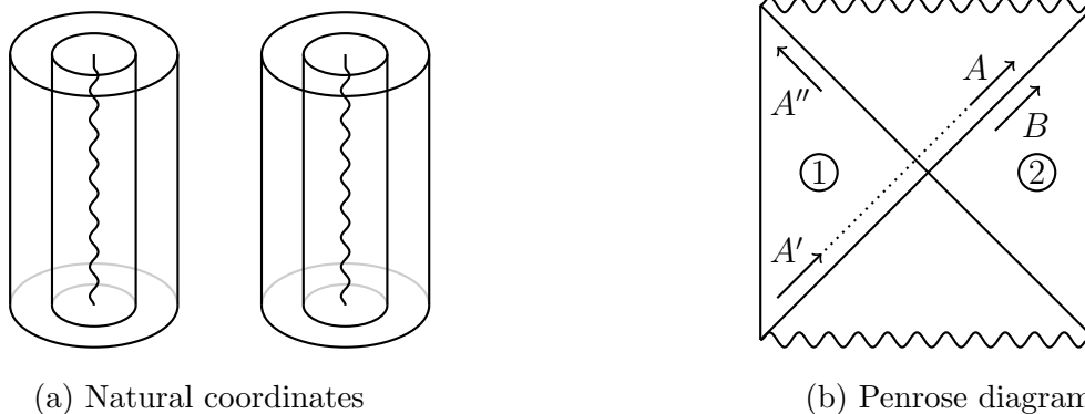
Figure 1: The extended black hole in anti-de Sitter space
