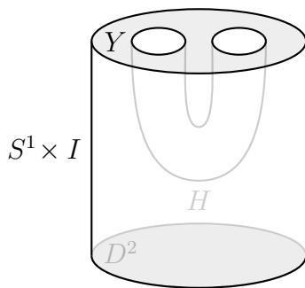
Figure 4: Cobordism from disk to disk with handle attached
