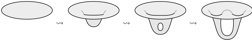
Figure 3: Formation of a wormhole
