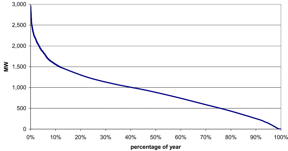
Fig. 2. VRE duration curve for Western Downs, Queensland, 2017.
