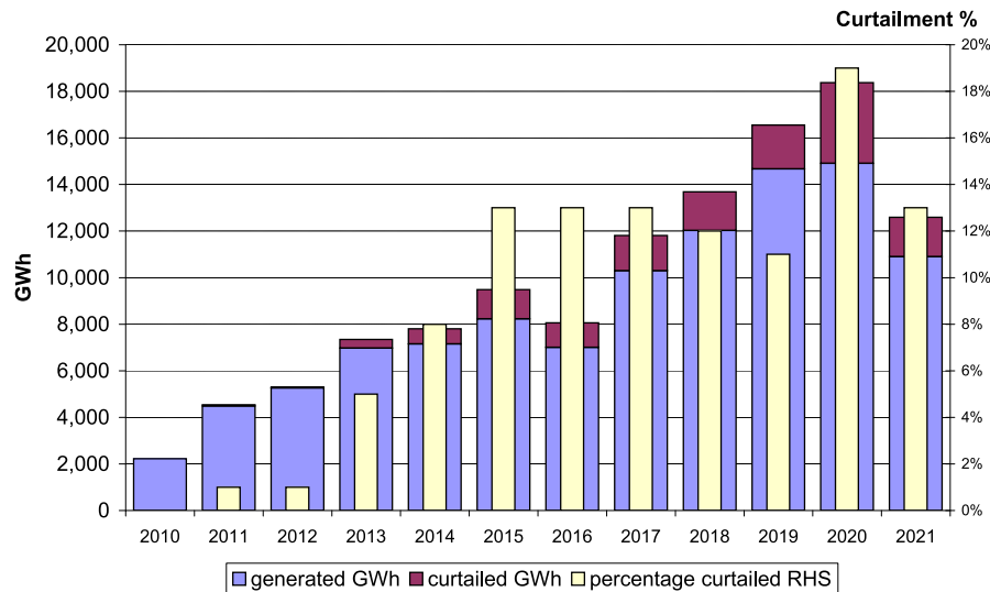
Fig. 1. Evolution of wind output and curtailment in Scotland, 2010–2021.
