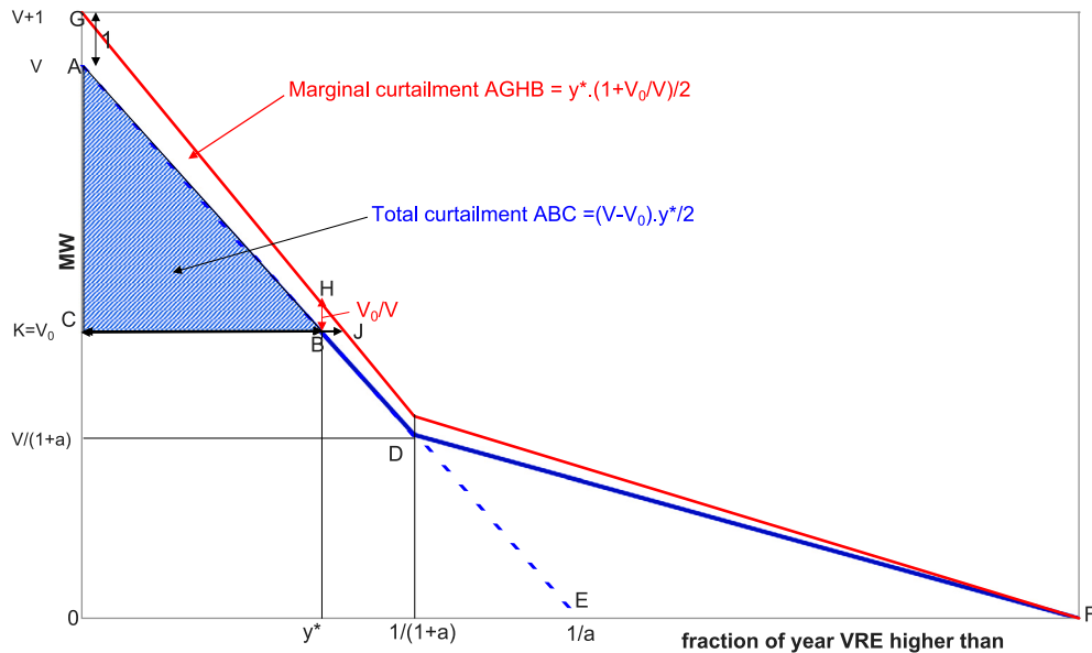
Fig. 3. Geometric illustration of average and marginal curtailment.
