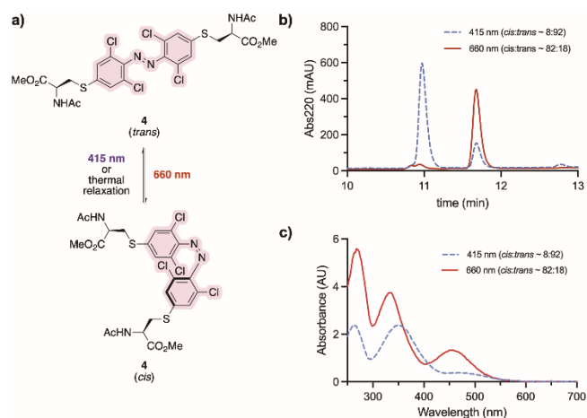
Figure 2. a) Photoisomerisation studies of cysteine-conjugated staple 4 . (b) Trans-cis isomerisation of 4 (500 \mu\text{M} in \text{H}_2\text{O} / MeCN 50:50) followed by analytical HPLC. (c) Isomer UV-vis analysis of 4 (500 \mu\text{M} in \text{H}_2\text{O} / MeCN 50:50). The spectra were recorded upon 30 min and 90 min irradiation with 415 nm and 660 nm LED lights, respectively.
