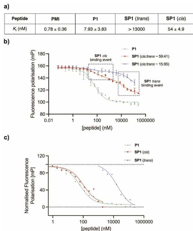
Figure 7. (a) Binding affinities of PMI, P1 and SP1 for MDM2. The K_i values are reported as the average of two or three biological replicates each performed as a triplicate and the error bars shown represent the standard error of the mean, determined from the fit for each of the independent experiments and subtracted from the average K_i value. (b) Competitive FP assay of P1 and SP1. Each data point is arithmetic mean of two two or three biological replicates each performed as a triplicate and the error bar shown are standard errors of the mean. In-situ isomerisation of SP1 was carried out upon 30 min and 90 min irradiation with 415 nm and 660 nm LED lights, respectively. (c) Normalised FP curves of cis and trans SP1 individual binding events, extracted from the SP1 ( cis:trans ~ 59:41) fitted curve, and the normalised FP of P1 for comparison.
