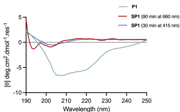
Figure 5. CD spectra of the linear peptide P1 in 50:50 H 2 O / MeCN, and stapled peptide SP1 in MeCN, recorded across 190–250 nm. In-situ isomerisation of SP1 was carried out upon 30 min and 90 min irradiation with 415 nm and 660 nm LED lights, respectively.
