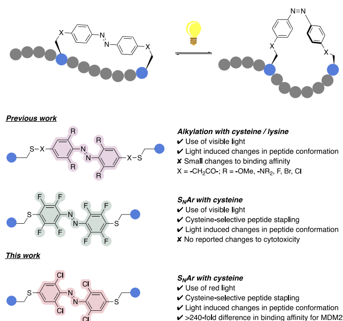
Figure 1. Previous work utilising alkylation and S N Ar for the incorporation of ortho -substituted ABs for peptide stapling, 14–19 together with our ortho -chloro AB red-light activated peptide stapling via Cysteine-S N Ar methodology.
