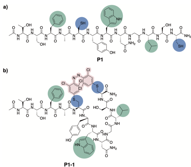
Figure 3. (a) Peptide stapling precursor P1 . Highlighted in blue the incorporated Cys residues and in green the amino acid residues involved in the interaction with MDM2. (b) Structure of the ( i , i +7) azobenzene-containing stapled peptide SP1 .
