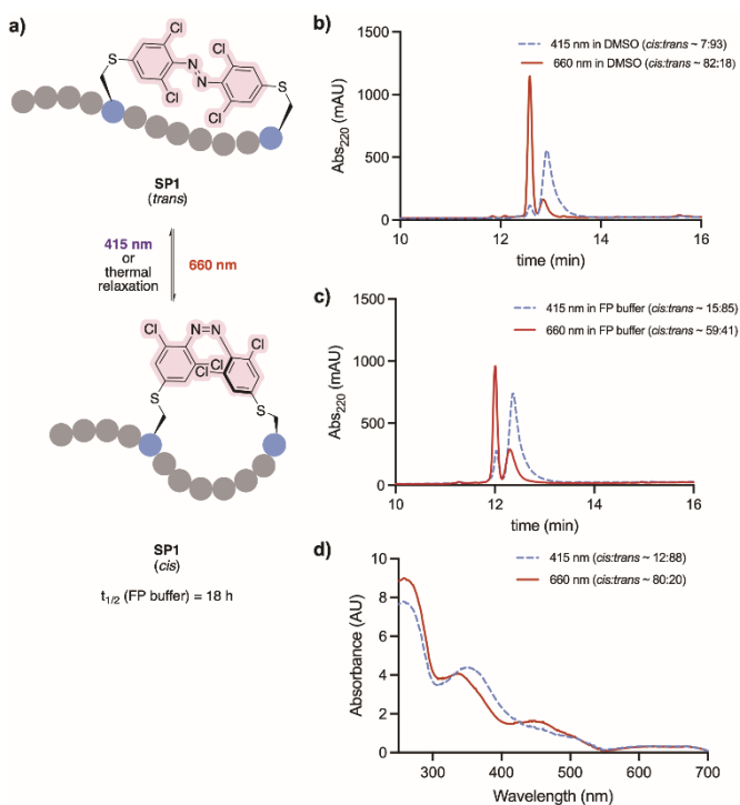
Figure 4. (a) Photoisomerisation of stapled peptide SP1 . (b) Trans-cis isomerisation of SP1 in DMSO followed by analytical HPLC. (c) Trans-cis isomerisation of SP1 in and FP buffer followed by analytical HPLC. (d) UV-vis spectrum of SP1 (500 \mu\text{M} \text{H}_2\text{O} / MeCN 50:50). All the spectra were recorded upon 30 min and 90 min irradiation with 415 nm and 660 nm LED lights, respectively.
