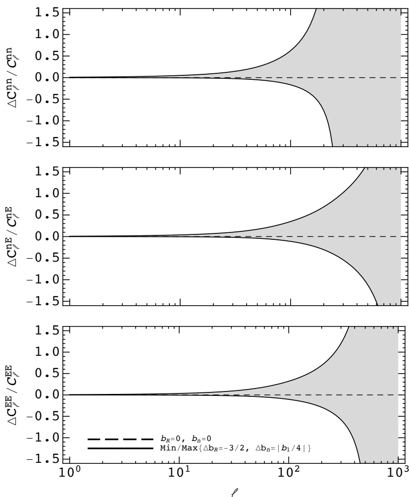
Figure 4. Relative one-loop bias contributions compared to the dark matter one-loop power spectra for C_\ell^{nn} , C_\ell^{nE} , C_\ell^{EE} . We again use b_1 = 1 , b_{R*} = -3/2 and for the rest of the biases we use the values |b_n| = b_1/4 . The sign of bias values b_n are adjusted so that the grey area represents the band of potential bias one-loop contributions where |b_n| < b_1/4 . In all cases we neglect the stochastic bias contributions. Effectively this gives an estimate of the validity regime of linear alignment model, provided our bias coefficient choice is realistic.
