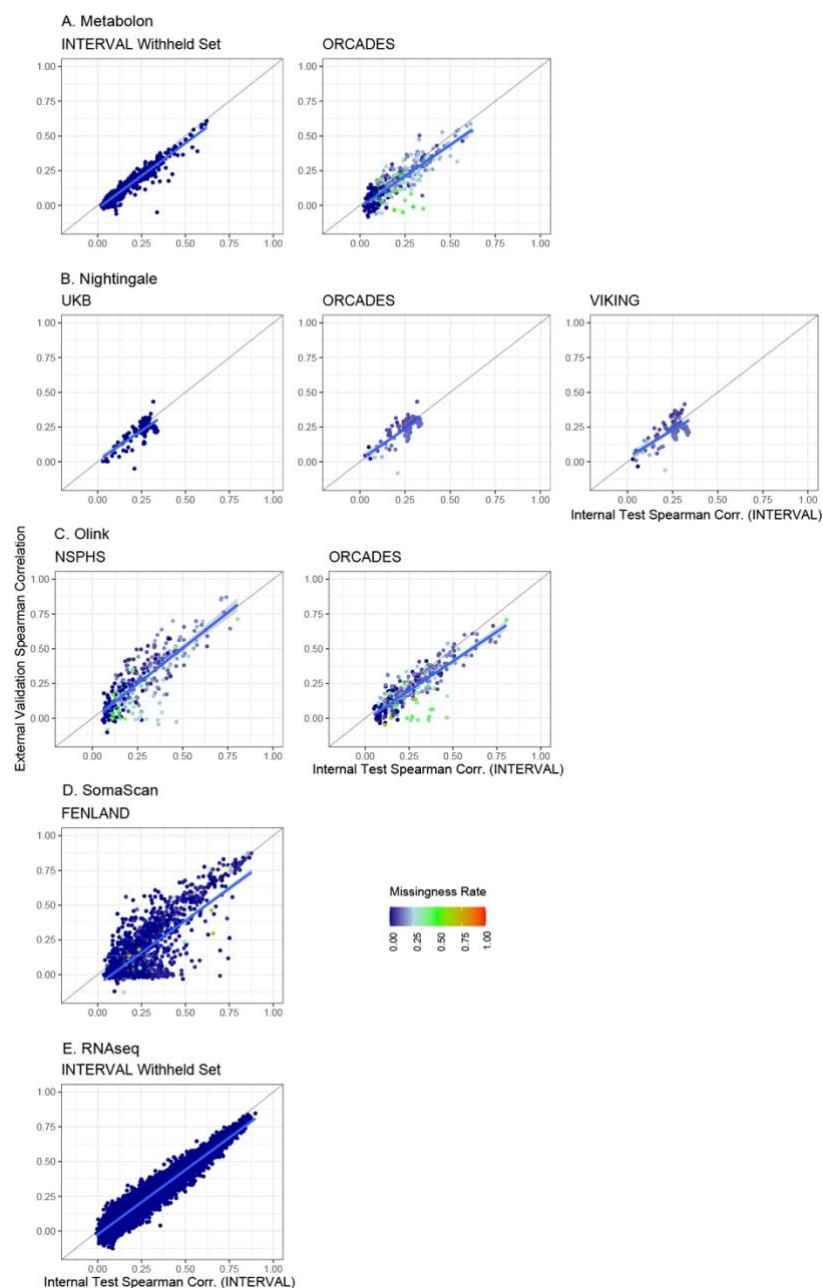
Extended Data Figure 4: Validation of genetic scores in external European cohorts. The scatter plots compare the spearman correlation scores between internal validation and external validation with a European cohort on each platform, in which points are coloured by the variant missingness rate in the external cohort and the blue line shows the linear models fitting the data points. This analysis included all the developed genetic scores in this study.
