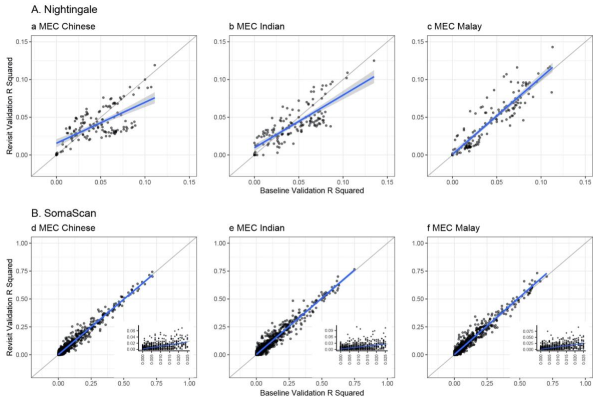
Extended Data Figure 7: Performance ( R^2 ) of genetic scores between longitudinal samples and across ancestries in the MEC cohort. Paired samples include a baseline and a revisit sample from each individual run on SomaScan and Nightingale for MEC Chinese (N=403 and 721 individuals), MEC Indian (N= 356 and 376) and MEC Malay (N=353 and 363). Blue lines denote linear models fitted to each set of data points and the shaded areas represent 95% confidence intervals where applicable. There is no Nightingale genetic scores with a R^2 > 0.15 in both internal and MEC validation, so (a, b, c) only show R^2 in the range of [0, 0.15] for clarity. The sub-box plots at the right bottom of (d, e, f) show the validation results of these traits with baseline validation performance ( R^2 ) between 0 and 0.025 in each ancestry.
