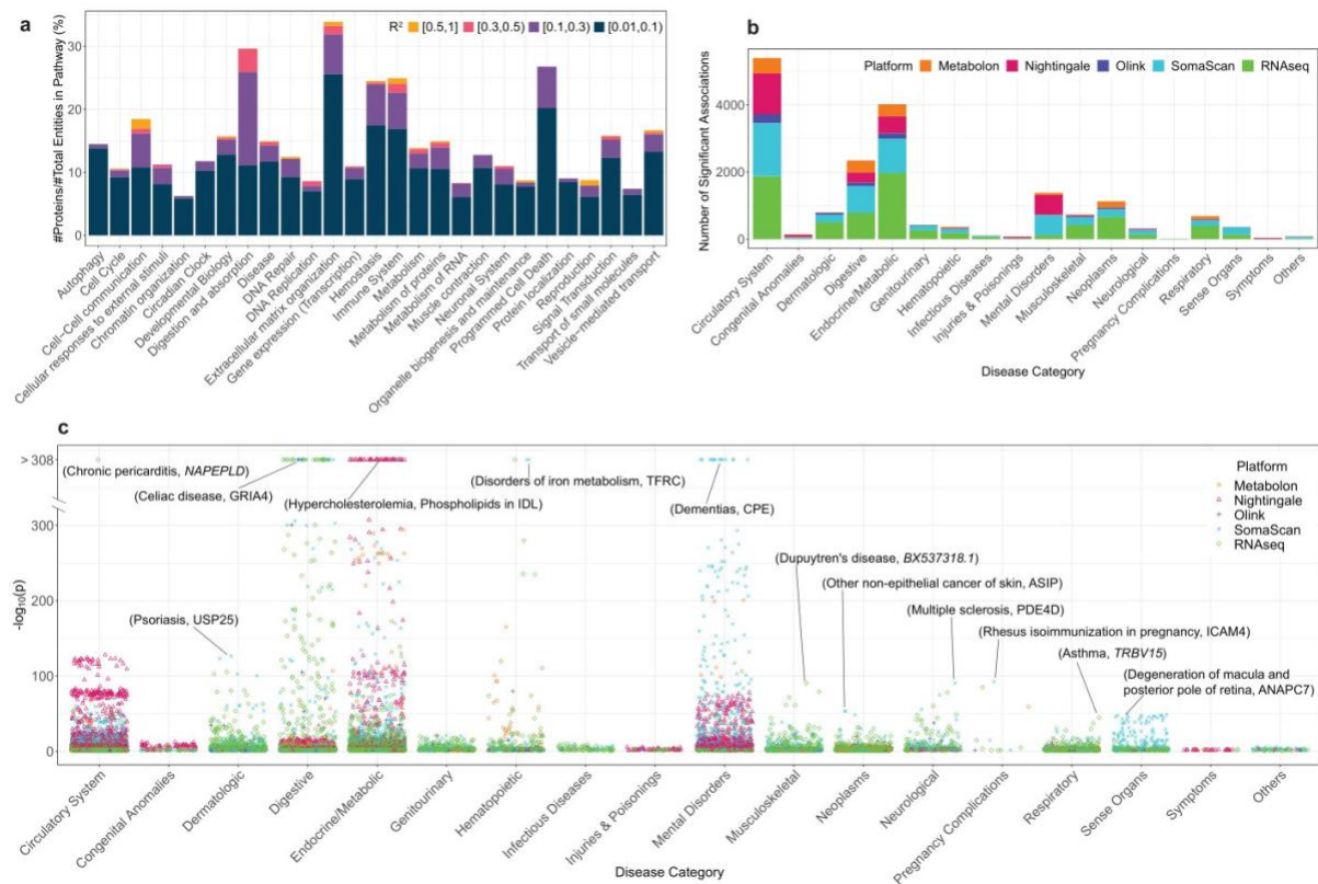
Figure 4: Applications of genetic scores of multi-omic traits. a , Genetic control of Reactome super-pathways using SomaScan and Olink genetic scores of varying R^2 in internal validation ( Methods ). b , Phenome-wide association study in UK Biobank. Stacked barplots show the number of detected significant associations by PheCode category of disease and omic platform (two-sided Wald test and FDR-corrected p-value < 0.05 for 11,576 tested traits). c , Strength of associations by category of disease and omic platform. Association with the lowest p-value for each disease category is labelled.
