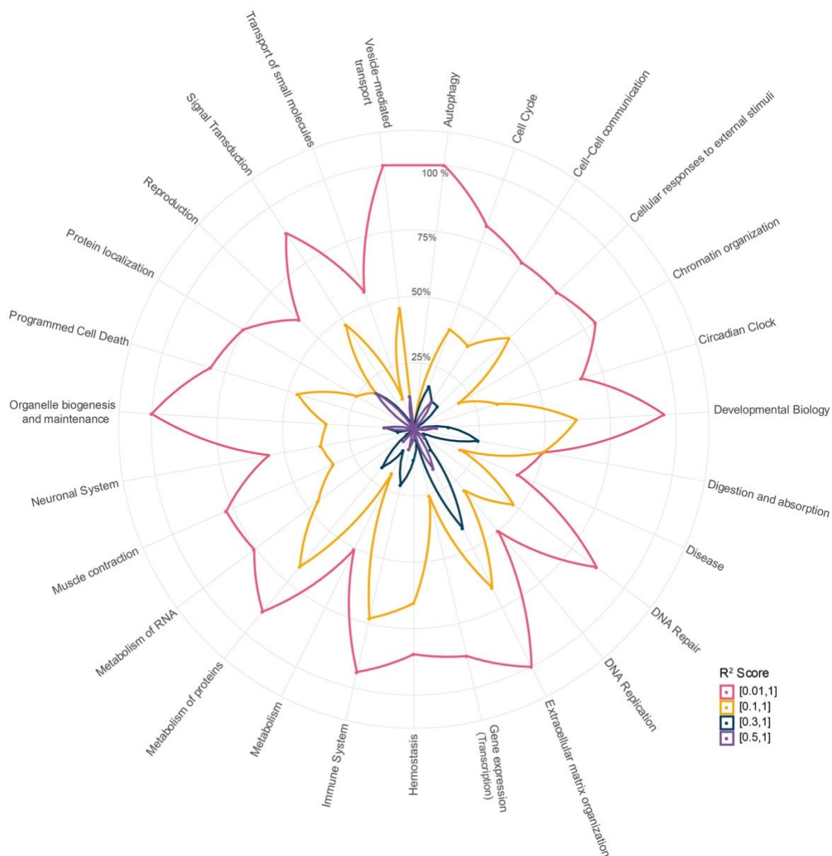
Extended Data Figure 8: Coverage analysis for blood proteins in the lowest-level pathways. This analysis looked at all the lowest-level pathways of super-pathways curated at Reactome. Where at least one protein genetic score are included in the entities of a lowest-level pathway, we consider this pathway is covered by proteins of this study. This figure shows the percentage of the lowest-level pathways a group of proteins (by R^2 in internal validation) covered among all the lowest-level pathways of each super-pathway.
