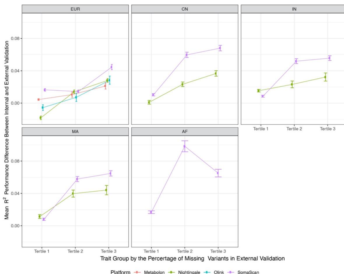
Extended Data Figure 5: Validation performance change of genetic scores by their variant missing rates in external cohorts of different ancestries. External validation results in European cohorts were merged in each platform to increase the statistical power in this analysis, which include NSPHS and ORCADES validations for Olink, and ORCADES and VIKINGS validations for Nightingale. Note that INTERVAL withheld subset validations and UKB validation for Nightingale traits were excluded in this analysis due to there is no or nearly no variant missingness in these external cohorts. Validation results in each platform were ranked by their variant missing rate of genetic score models in the external cohort and grouped into tertiles, where variant missing rate is the number of variants missing in the validation cohort / the total number of variants in the genetic score. This figure presents the mean and standard error (SE) of R^2 performance change of genetic scores between internal and external validation across tertiles of validation results. The analysis included validation results of 2,129 SomaScan, 603 Olink, 455 Metabolon and 423 Nightingale traits (traits can be overlapped for the same platform across multiple validation cohorts) for European (EUR); 2,047 SomaScan and 139 Nightingale traits for Chinese (CN), Indian (IN) and Malay (MA); 820 SomaScan traits for African American (AF).
