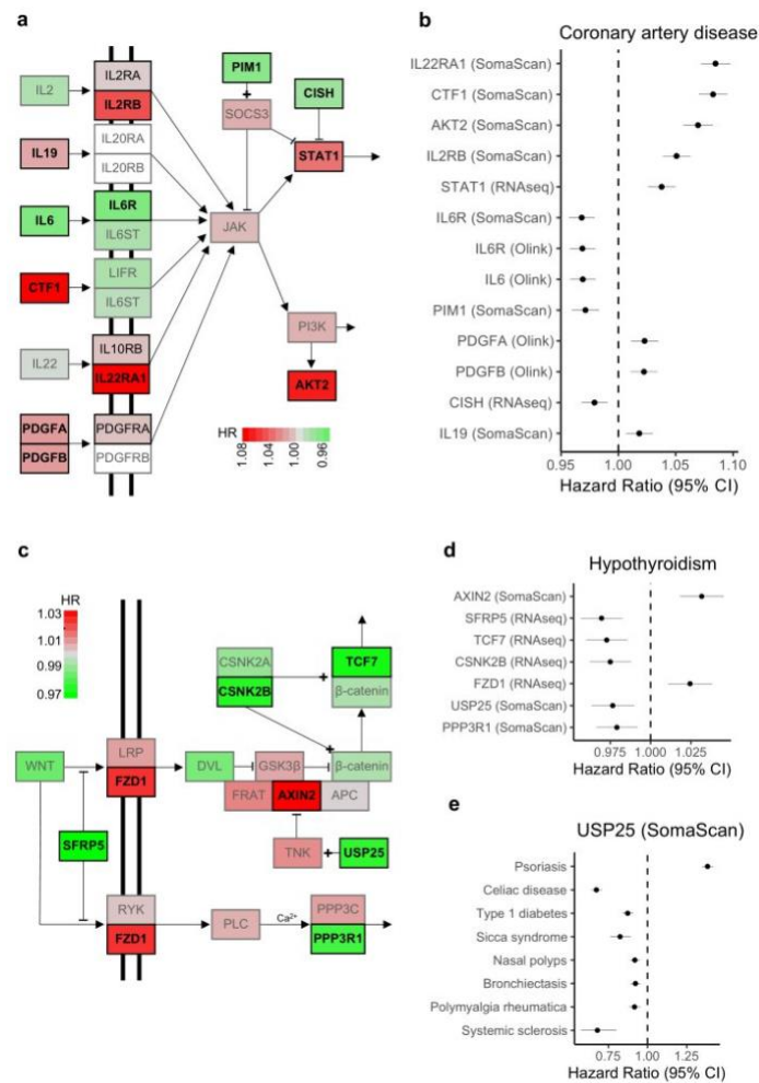
Figure 5: JAK/STAT and Wnt signalling pathways. a, c, Pathway diagrams for (a) JAK/STAT and (c) Wnt signalling. Nodes coloured based on hazard ratio (HR) of the genetic score for (a) coronary artery disease (CAD) and (c) hypothyroidism. Nodes are white if there is not a corresponding genetic score. The most significant HR across omic platforms is used at each node. Nodes are bold if the genetic score had FDR-adjusted p-value < 0.05 (two-sided Wald test and correcting for 11,576 tested traits). b, d, Forest plots of FDR-significant HRs for (b) CAD (n = 28,854 cases and 390,159 controls) and (d) hypothyroidism (n = 21,871 cases and 404,440 controls) for genetic scores in (b) JAK/STAT or (d) Wnt signalling. e, Forest plot of HRs and 95% confidence intervals for the genetic score of USP25 (SomaScan) across multiple diseases.
