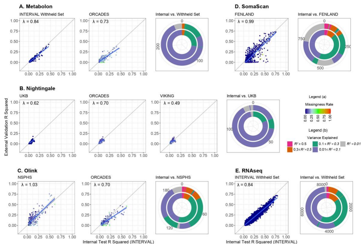
Figure 2: External validation of genetic scores in cohorts of European ancestry.
