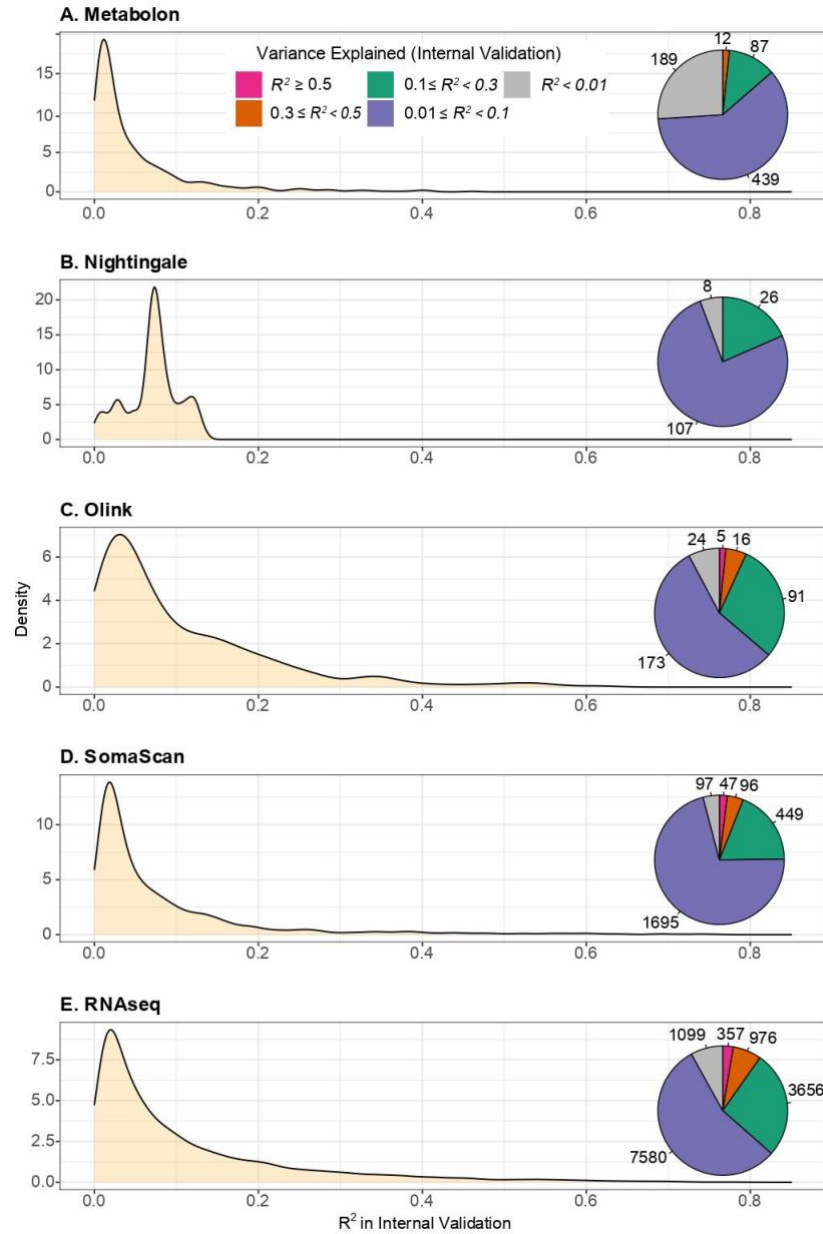
Figure 1: Performance of multi-omic genetic scores in internal validation. The variance explained in the measured biomolecular trait ( R^2 ) by the genetic score is assessed in the internal validation set of INTERVAL ( Methods ). Pie charts reflect the number of genetic scores in a particular R^2 range.
