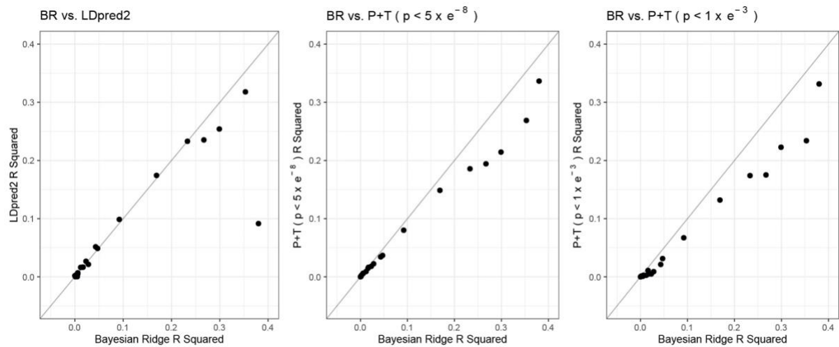
Extended Data Figure 2: R^2 performance comparison between Bayesian ridge, LDpred2, P+T for Metabolon traits in external validation (INTERVAL withheld set). This figure compares the R^2 performance between BR (on the set of genome-wide variants with p -value < 5 \times 10^{-8} ; x-axis) and LDpred2 (Hapmap3 variant set), and between BR and P+T (variant sets of two p -value thresholds: 5 \times 10^{-8} and 1 \times 10^{-3} ) for 20 randomly selected Metabolon traits in external validation (INTERVAL withheld set; Methods ). P -values in the GWAS for omic traits were derived by t-test in linear regression and all tests were two-sided.
