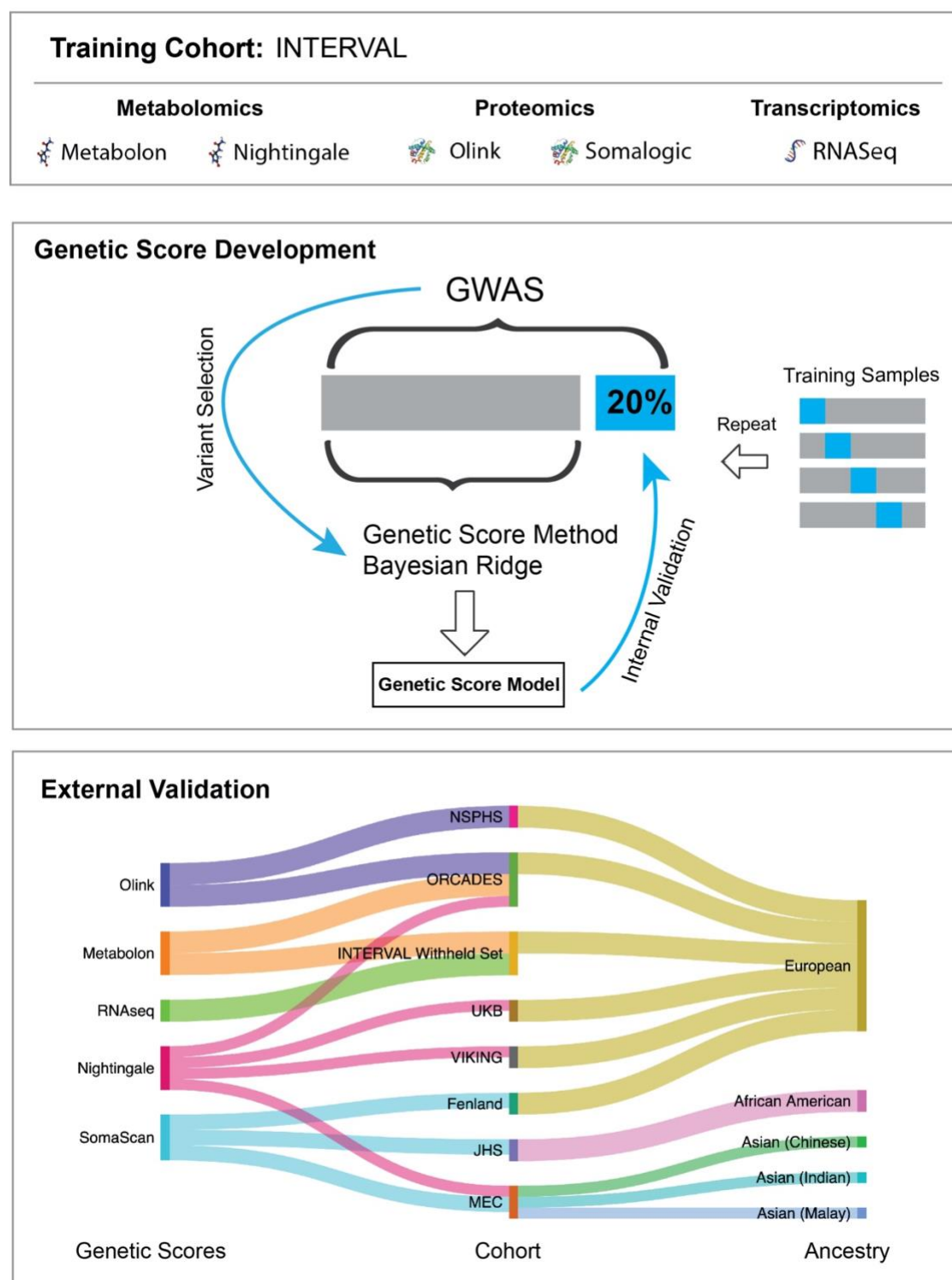
Extended Data Figure 1: Schematic framework for the development and validation of multi-omic genetic scores. This figure presents the overall study design for the development of genetic scores for multi-omic traits across five platforms (Nightingale, Metabolon, Olink, SomaScan and RNAseq) using INTERVAL data as well as their validation in seven external cohorts of multiple ancestries (European, Asian-Chinese, Asian-Malay, Asian-Indian and African American).
