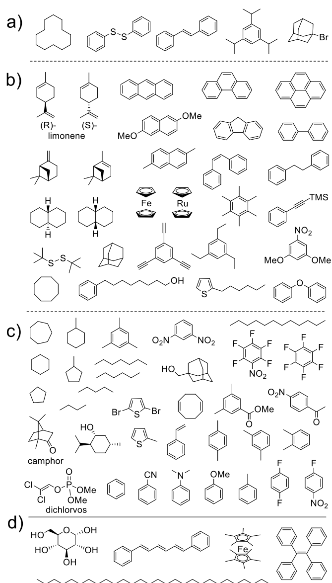
Figure 2. Prospective guest molecules for host \Delta\Delta\Delta\Delta - 5 : a ) larger hydrophobic guests that bound weakly (slow exchange by NMR); b ) medium-sized hydrophobic guests that bound strongly (slow exchange by NMR); c ) smaller guests for which fast exchange was observed; d ) compounds that were not encapsulated.
