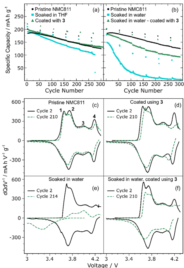
Fig. 5 (a and b) Long-term electrochemical cycling data (specific discharge capacity/ \text{mA h g}^{-1} vs. cycle number). (a) Results for the pristine PC-NMC811, PC-NMC811 coated using 3 and control uncoated sample. (b) Results of PC-NMC811 soaked in water with and without a further coating step. These electrochemical measurements were carried out in half cell configuration (vs. Li) between 3 and 4.3 V. The cycling was performed at C/2 rate and slow C/20 cycles were included every 50 cycles. (c–f) dQ/dV profiles measured for the slow (C/20) cycles of PC-NMC811 samples. (c) Pristine PC-NMC811, (d) PC-NMC811 coated with 3 , (e) PC-NMC811 soaked in water and then annealed at 400 °C under air. (f) PC-NMC811 soaked in water, coated with 3 and annealed under air at 400 °C.
