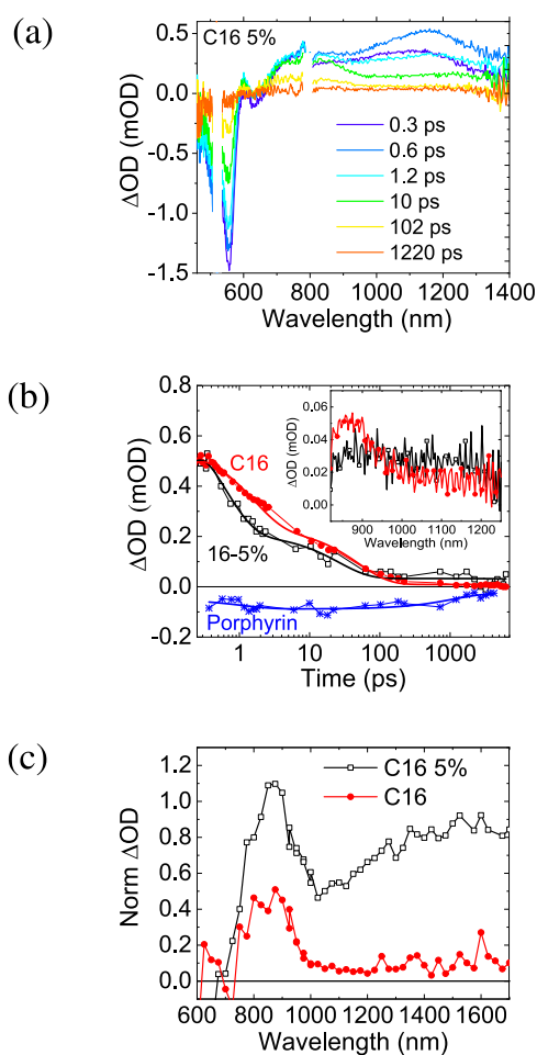
Figure 4. Transient absorption spectra of thin films of (a) C_{16} -5%, recorded using a 525 nm excitation pulse. (b) Decay of S_1 excited-state absorption in C_{16} and C_{16} -5% (red and black, respectively), probed at 1270 nm, and the Pd porphyrin bleach dynamics in C_{16} -5% (blue). The inset presents the average transient absorption spectrum at 2–4.7 ns in the near-infrared identifying excited-state population differences between C_{16} (red) and C_{16} -5% (black). (c) Transient absorption spectra at 1 \mu s normalized per photon absorbed of C_{16} (red, circles) and C_{16} -5% (black, open squares), obtained with 520 nm excitation with an excitation density of 40 \mu\text{J}/\text{cm}^2 . For the decays, band-pass filters were used to avoid the white light effect.
