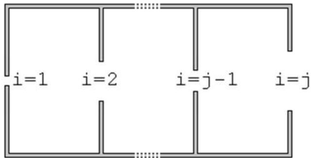
Figure 4: A series of openings whose areas can be described by a single effective area, A_{eff} .
