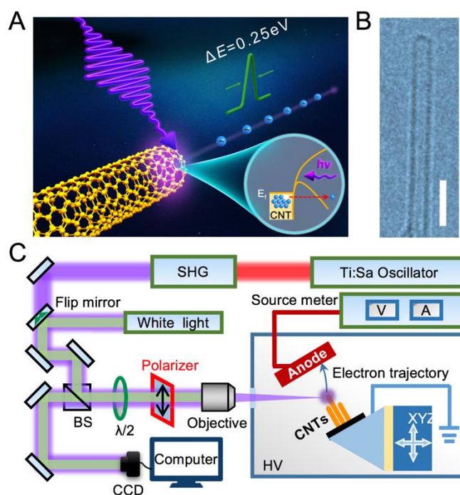
Figure 1. Highly coherent CNT-based photoemission source. (A) Emission dynamics. (B) High-resolution transmission electron microscopy image of a typical CNT under study. Scale bar: 5 nm. (C) Experimental setup. (SHG, second harmonic generation. CCD, charge-coupled device. BS, beam splitter. HV, high vacuum.)
