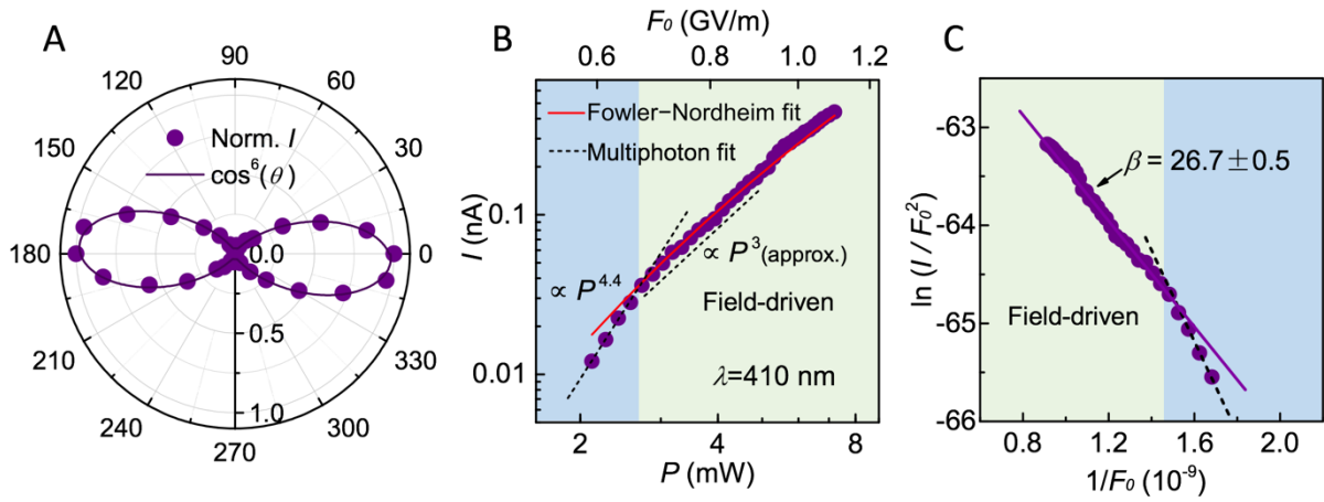
Figure 2. Field-driven photoemission at 410 nm pump wavelength. (A) Normalized emission current ( I ) as a function of the angle of polarization ( \theta ) of the input optical source. Note the emission currents show a \cos^6(\theta) dependence. (B) Emission current as a function of laser power ( P ) (bottom abscissa) and laser field ( F_0 ) (top abscissa) at bias voltage ( V_b ) of 50 V. At low power range, multiphoton regime is noted, while field-driven regime is noted at higher power range. (C) FN plot of the optically driven emission current, showing a field enhancement factor ( \beta ) of 26.7 \pm 0.5 . Green area in (B) and (C) corresponds to the field-driven regime region. \lambda , wavelength.
