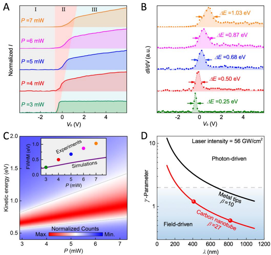
Figure 3. Electron beam characterization. (A) Dependence of the normalized emission current on bias voltage ( I - V_b ) at different laser powers ( P ). Stage I: fully retarding region; stage II: fast collecting region; stage III: beam focusing region. (B) corresponding dI/dV curves; the width of the peaks (FWHM) indicates the energy spreads ( \Delta E ), while the shoulder indicates the beam divergence grade. (C) Contour plot representation of the normalized counts as a function of P and kinetic energy, according to the extended Simpleman model. The FWHM is marked as the range between upper and lower dotted lines. The inset shows FWHM of the
