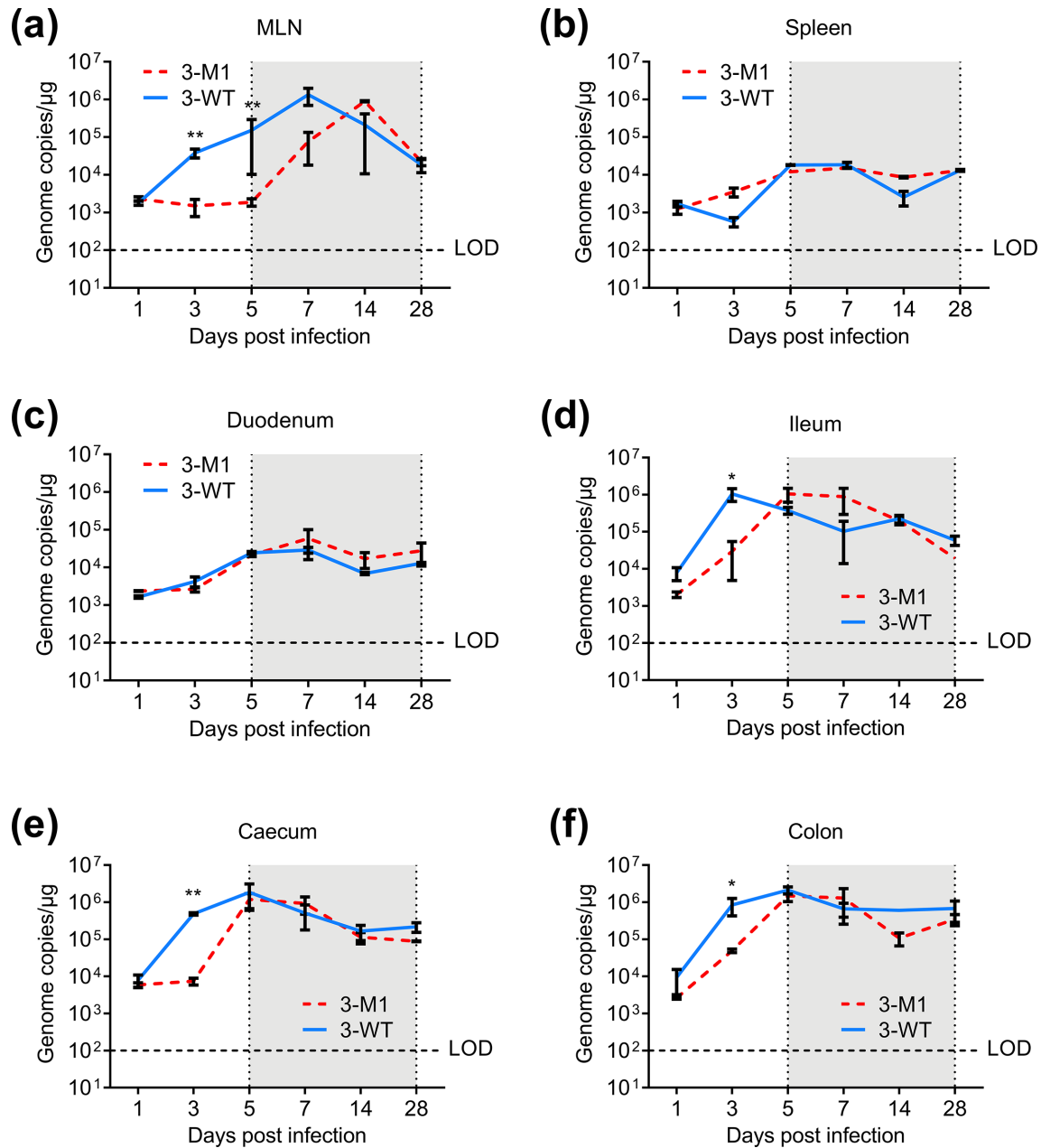
Fig. 5. Replication kinetics in tissues. C57BL/6 mice were orally gavaged with 1000 TCID 50 of WT MNV-3 (3-WT) or MNV-3 M1 (3-M1). Mock inoculated mice were treated with DMEM. vRNA was extracted from tissue samples, including (a) MLN, (b) spleen, (c) duodenum, (d) ileum, (e) caecum and (f) colon, and quantified using qPCR. Statistical analyses were carried out using an unpaired t -test. For WT MNV-3, n =20; for MNV-3 M1, n =20; and for mock, n =5. Shaded area shows the time points from which reversion was seen. * P ≤0.05; ** P ≤0.01. LOD, limit of detection.
