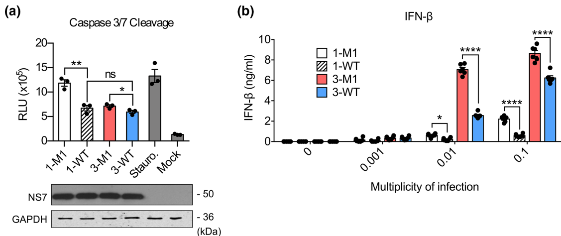
Fig. 3. VF1 delays apoptosis and inhibits IFN induction in MNV-3-infected cells. (a) BALB/c BMDMs were infected at an m.o.i. of 5 TCID 50 per cell with WT MNV-1 (1-WT), MNV-1 M1 (1-M1), WT MNV-3 (3-WT) or MNV-3 M1 (3-M1), or treated with staurosporine or DMEM. Caspase 3/7 activity was assayed in triplicate 15 h post-inoculation (top panel). Statistical analysis was carried out using an unpaired t -test. Lysates were analysed by western blotting (bottom panel). RLU, relative luminescence unit. (b) RAW264.7 cells were infected with the indicated viruses at different m.o.i. Supernatant was harvested 24 h post-infection and assessed by ELISA. Two-way ANOVA with Bonferroni multiple comparisons tests was used to determine statistical significance. ns= P>0.05 ; * P\leq 0.05 ; ** P\leq 0.01 ; **** P\leq 0.0001 . ns, Not significant.
