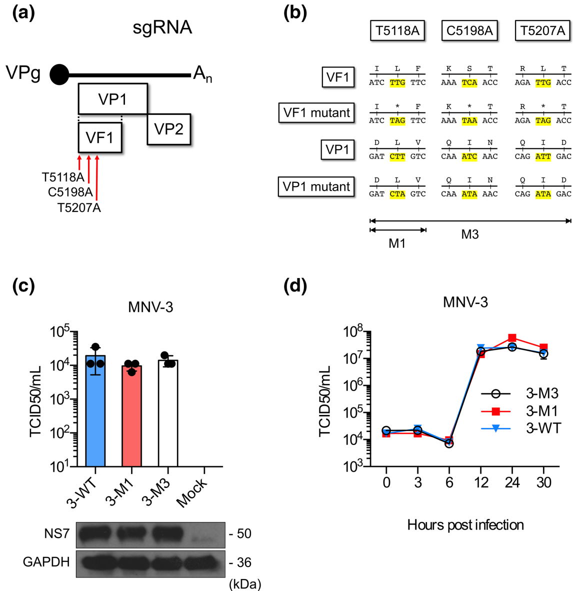
Fig. 2. MNV-3 VF1 is dispensable for replication in cell lines. (a, b) Schematic representations of the MNV subgenomic RNA indicating sites of stop codon placements for MNV-3 M1 and MNV-3 M3. Stop codon mutations are nonsense for VF1 as they introduce stop codons at position 5118 for MNV-3 M1, and at 5118, 5198 and 5207 for MNV-3 M3. (c) Plasmids encoding full-length WT MNV-3 (3-WT), MNV-3 M1 (3-M1) or MNV-3 M3 (3-M3) were transfected into BSRT7 cells. Recovered viruses were titrated in BV-2 cells (top panel). Antisera to NS7 and GAPDH were used for western blot analysis (bottom panel). (d) Single-step growth curve analysis. BV-2 cells were infected at an m.o.i. of 5 TCID 50 per cell with WT MNV-3 (3-WT), MNV-3 M1 (3-M1) or MNV-3 M3 (3-M3). Samples were harvested at 0, 3, 6, 12, 24 and 30 h post-infection. Viruses were titrated in triplicate in BV-2 cells.
