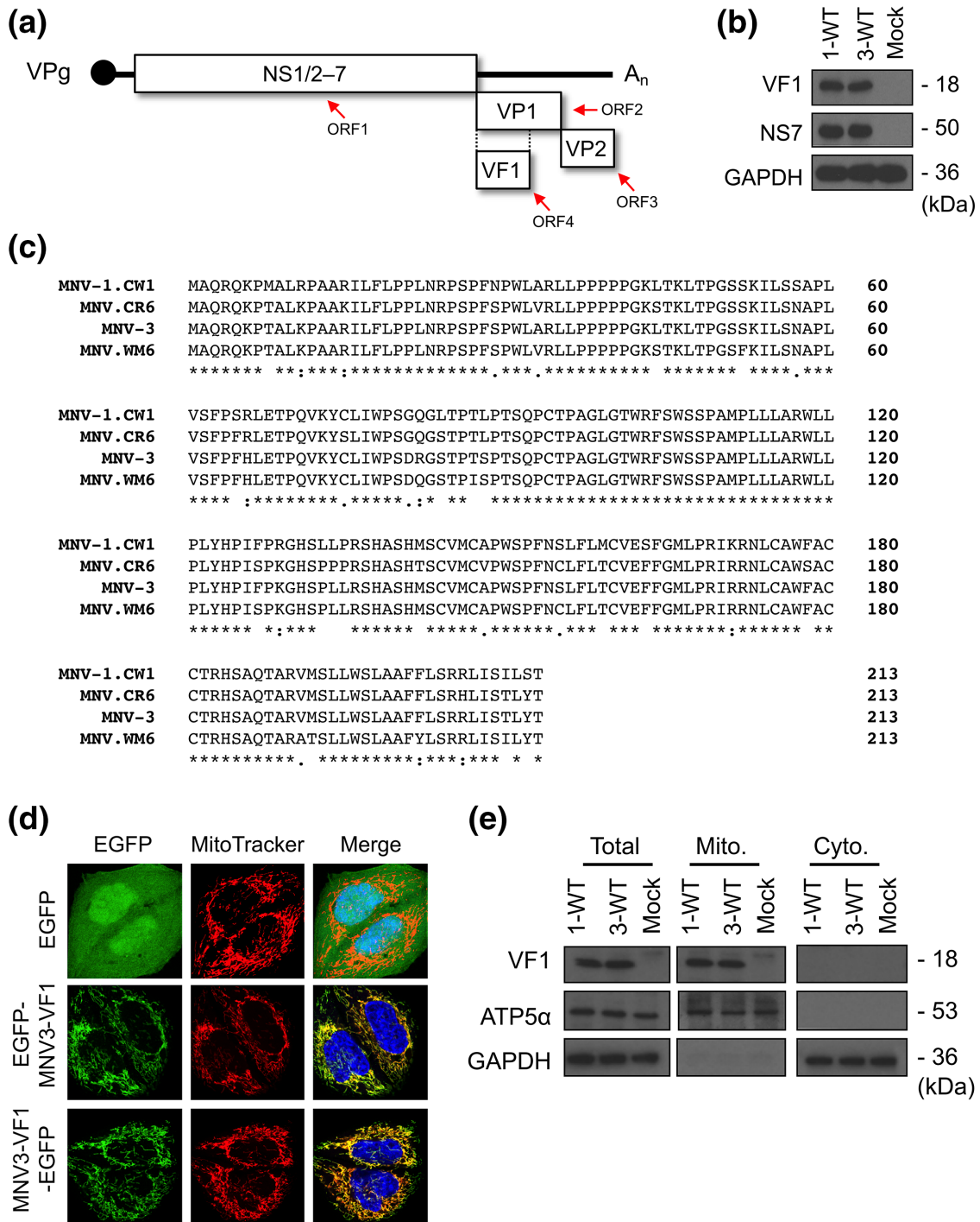
Fig. 1. In vitro characterization of MNV-3 VF1. (a) A schematic representation of the MNV genome, showing the four ORFs that encode the non-structural proteins NS1/2-7, VP1, VP2 and VF1. (b) Western blot analysis of VF1 expression following a 12 h infection with MNV-1 (1-WT) and MNV-3 (3-WT) in RAW264.7 cells (m.o.i.=5). Mock inoculated samples were treated with Dulbecco's modified Eagle medium (DMEM). (c) An alignment of VF1 protein sequences from MNV-1 (acute, lab-adapted strain), MNV-3 (persistent, lab-adapted strain), CR6 (persistent, lab-adapted strain) and WM6 (persistent, wild strain). VF1 encoded by MNV-3 and MNV-1 are 89% identical. (d) Confocal microscopy of MEFs transfected with plasmids expressing enhanced green fluorescent protein (EGFP), or EGFP fused to the N or C terminus of MNV-3 VF1. Green indicates EGFP, red indicates MitoTracker and blue denotes DAPI. (e) Biochemical fractionation of BV-2 cells infected with MNV-1 (1-WT) and MNV-3 (3-WT) (m.o.i.=5). Mock inoculated cells were treated with DMEM. Lysates were collected 12 h post-infection and mitochondrial (mito.) and cytoplasmic (cyto.) fractions were enriched as described in the text.
