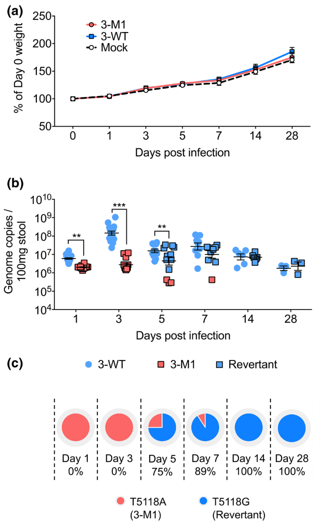
Fig. 4. Analysis of MNV-3 VF1 virulence in vivo . C57BL/6 mice were orally gavaged with 1000 TCID 50 of WT MNV-3 (3-WT) or MNV-3 M1 (3-M1). Mock inoculated mice were treated with DMEM. (a) Weights of mice are presented as relative to their day 0 weights ( n=8 ). (b) vRNA extracted from faecal samples was quantified using qPCR. Points shaded blue represent VF1 expression (either from WT or revertant viruses). Red points represent absence of VF1 expression. Statistical analyses were calculated using two-way ANOVA with Bonferroni post-tests. (c) Percentages of mice that are shedding revertant viruses after acquiring the A5118G substitution. ** P \leq 0.01 ; *** P \leq 0.001 .
