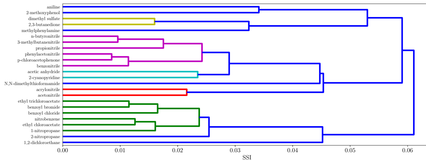
Figure S9: Dendrogram for solvents to the left of node 9 in Figure 2.
