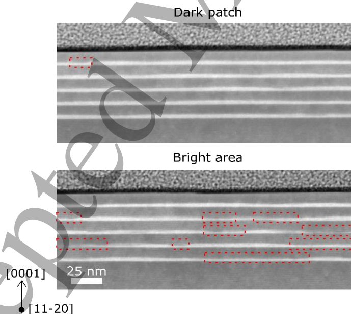
Figure 7 STEM HAADF images showing the MQW structure of the dark patch and the bright area in the sample grown at 698 °C. The bright lines show the positions of QWs. GWWFs are marked in red dotted boxes. The material above the dark line is the Pt protective layer.
