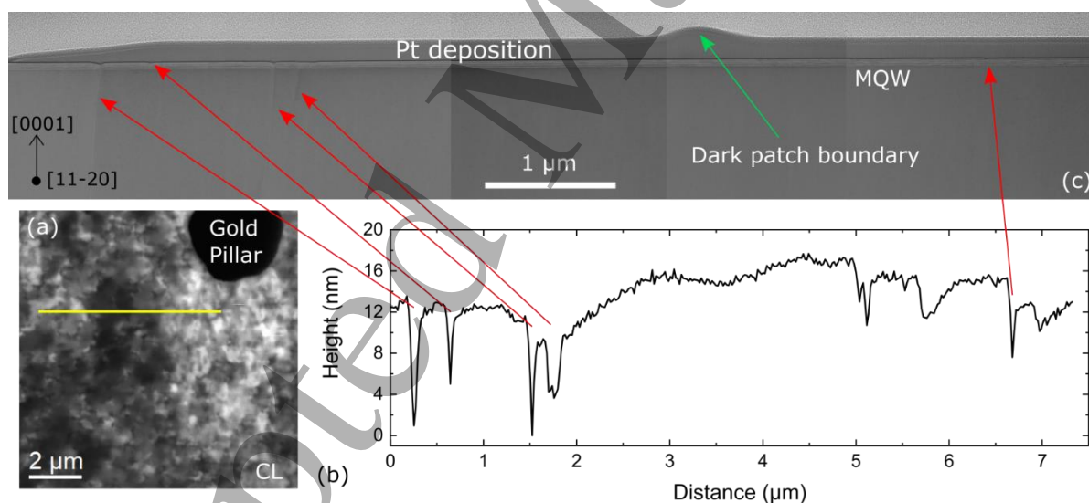
Figure 6 (a) The CL image taken in step 2. The line-scan position is highlighted by the yellow line. (b) The AFM profile corresponding to the line-scan position extracted from the AFM image taken in step 4. (c) The overview STEM HAADF image taken in step 6. Dislocations in (c) are matching with the dislocation pits found in (b). The dark patch boundary found in step 3 is marked by thicker Pt deposition on the sample surface, which is highlighted by the green arrow.
