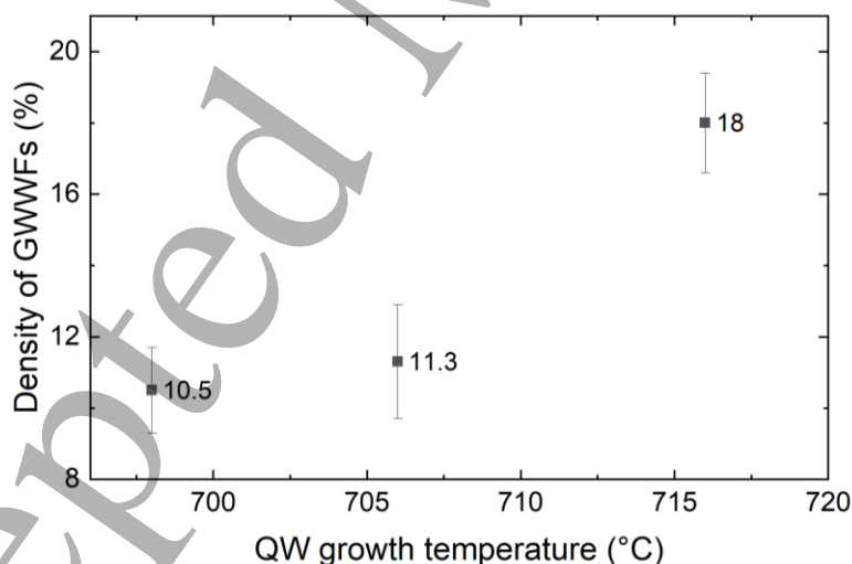
Figure 8 The average densities of GWWFs plotted against the QW growth temperatures
