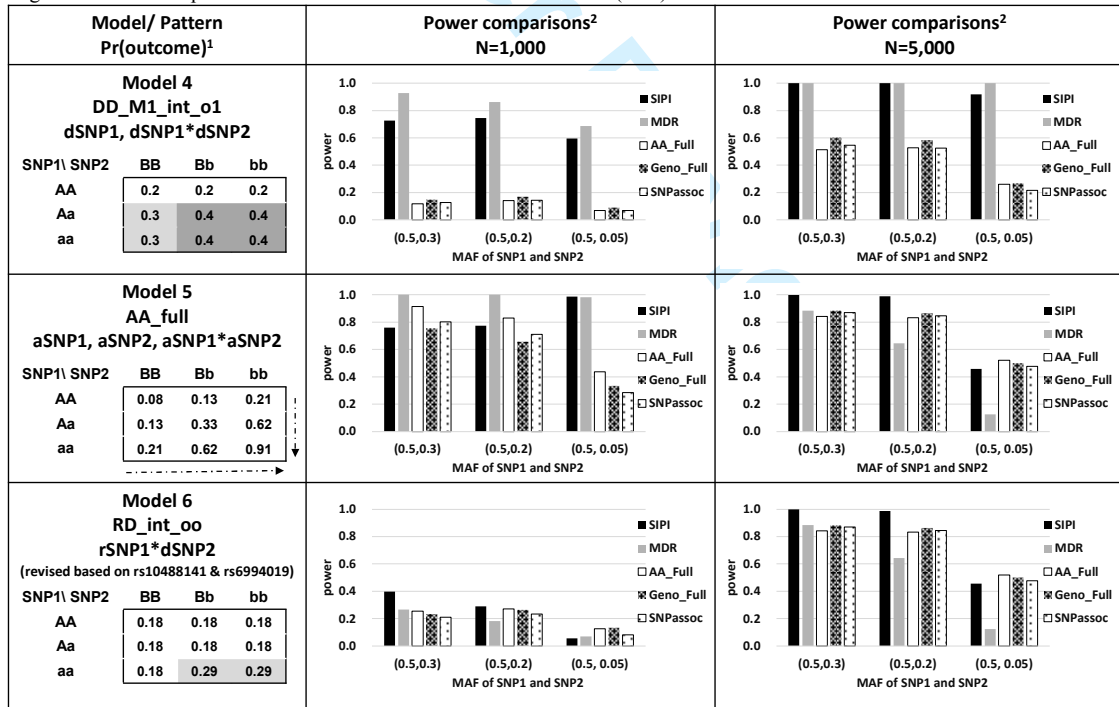
Figure 2. Power comparisons of the SNP Interaction Pattern Identifier (SIPI) and other four methods for Models 4-6
