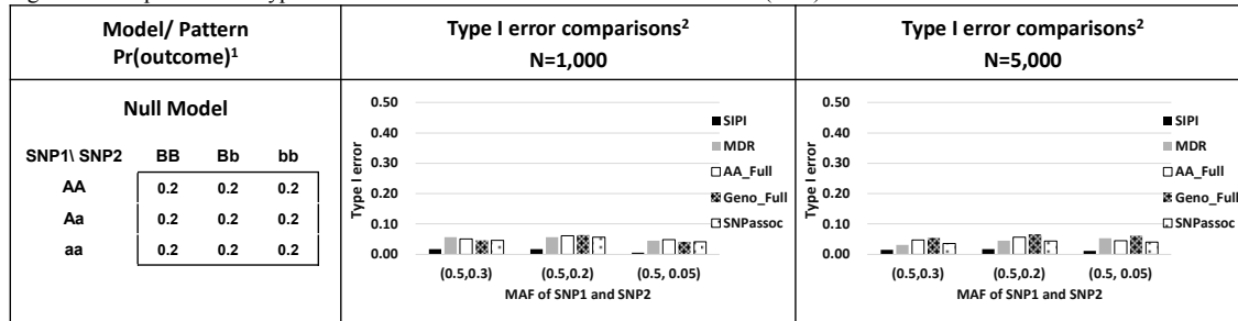
Figure 3. Comparisons of Type I errors of the SNP Interaction Pattern Identifier (SIPI) and other four methods
