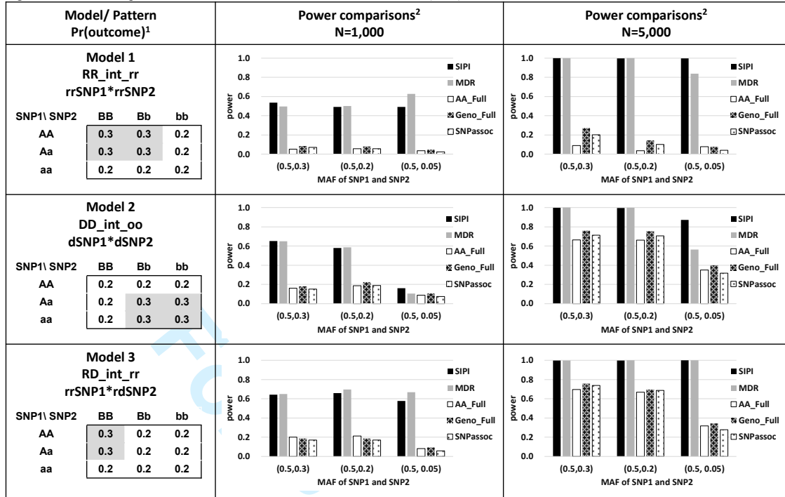
Figure 1. Power comparisons of the SNP Interaction Pattern Identifier (SIPI) and other four methods for Models 1-3
