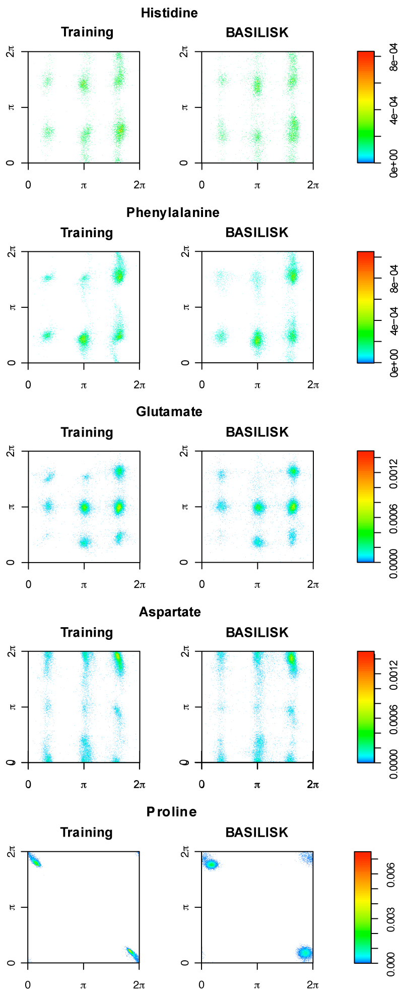
Additional figure 4: \chi_1 versus \chi_2 histograms for histidine, phenylalanine, glutamate, aspartate and proline. Histograms marked “Training” were generated from the training set; histograms marked “BASILISK” were generated from BASILISK samples.
