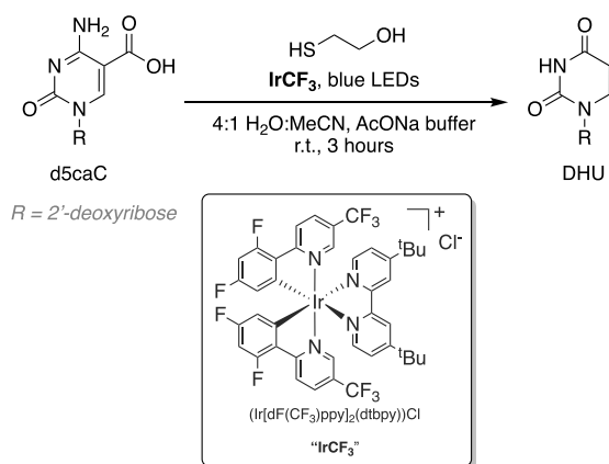
Figure 2. Photocatalytic conversion of 5-carboxycytidine to 5,6-dihydrouacil.
