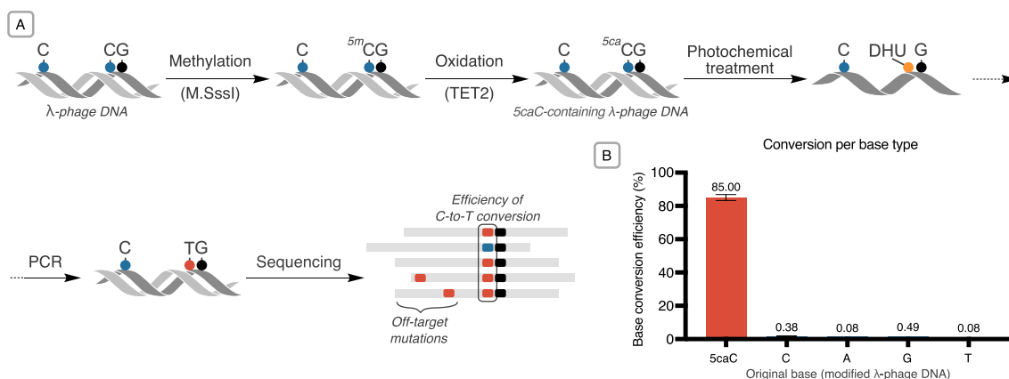
Figure 6. (A) Modified λ-phage DNA was subjected to various photochemical conditions and the results evaluated via next-generation sequencing. (B) Barplot of mean base conversion rates (±std deviation, n = 2) resulting from photochemical treatment of the modified genome (0.5 M thioglycerol, 0.1 mM photocatalyst, 20 min illumination followed by 2 h hydrolysis at 37 °C; Table S6, entry 8). The rate of on-target 5caC-to-T transitions observed at CpG sites during base calling was corrected to account for unmethylated and unoxidized bases.
