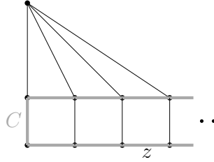
Figure 1: The dominated ladder is obtained from the one ended ladder by adding a vertex that is adjacent to every vertex on the upper side of the ladder. The topological cycles of VTOP of the dominated ladder do not induce a matroid as they violate the elimination axiom (C3): We cannot eliminate all the triangles from the grey cycle C .
