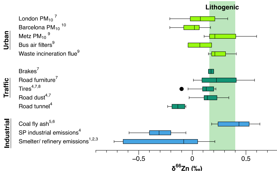
Fig. 6. Plot of \delta^{66}\text{Zn}_{\text{JMC}} values for anthropogenic reservoirs. SP refers to the city São Paulo. Green vertical shaded area gives range of lithogenic values for Zn +0.28 \pm 0.12\text{‰} from (Moynier et al., 2017). References: 1. (Mattioli et al., 2009), 2. (Bigalke et al., 2010), 3. (Gelly et al., 2019) 4. (Souto-Oliveira et al., 2018), 5. (Borrok et al., 2010), 6. (Novak et al., 2016), 7. (Dong et al., 2017), 8. (Thapalia et al., 2010), 9. (Cloquet et al., 2006a) 10. (Ochoa et al., 2016). (For interpretation of the references to colour in this figure legend, the reader is referred to the web version of this article.)
