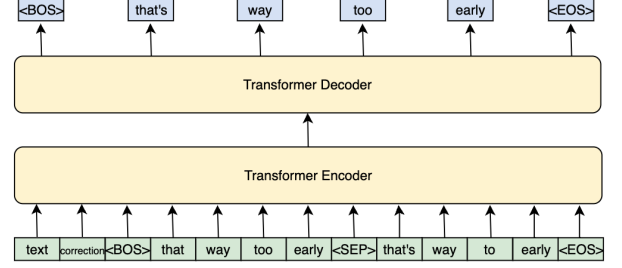
Figure 2: Model structure of N-best T5.
