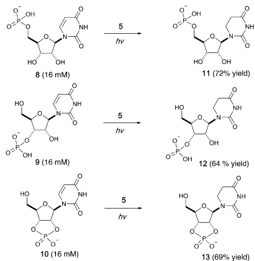
Fig. 2 Photoreduction of uridine nucleotides to dihydrouridine nucleotides. Yields are based on relative integration of the signals in 1 H NMR spectra compared to an internal standard (sodium succinate).
