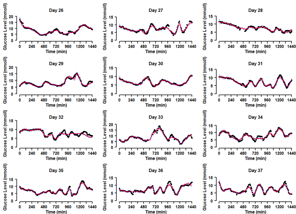
Fig. 2. Model fit of CGM data in a sample subject Cam03 (Day 26 – Day 37 are shown). The black circles are CGM measurements, the red solid lines represent the median of model fit, and the blue dashed lines represent 95% credible intervals of model fit.
