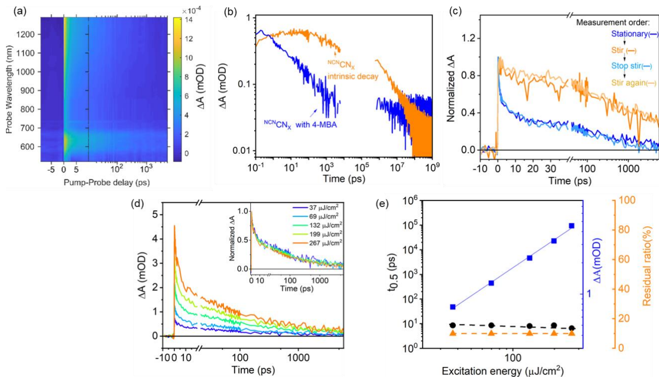
Figure 3. Electron accumulation in \text{NCN}\text{CN}_x induced by the addition of 4-MBA, as measured by its impact on the electron decay kinetics. (a) Transient absorption spectra of \text{NCN}\text{CN}_x in the presence of 4-MBA (10 mM) at different time delays after excitation at 355 nm. (b) Comparison of the corresponding electron decay kinetics measured at 680 nm with and without 4-MBA. The kinetic traces over 9 orders of magnitude from fs to ms are obtained by combining both ultrafast and microsecond TAS measurements excited at the same laser intensity. (c) Effect of stirring on the electron decay kinetics of \text{NCN}\text{CN}_x in the presence of 10 mM 4-MBA. Measurements are conducted in the following orders: Stationary, with stirring, stop stirring and then stirring again. Stirring had no effect on equivalent data for the \text{NCN}\text{CN}_x sample without 4-MBA (Figure S13). Data measured at \sim 69 \mu\text{J}/\text{cm}^2 (d) Fluence dependent electron decay kinetics of \text{NCN}\text{CN}_x in the presence of 4-MBA, measured without stirring. Inset graph: the normalized kinetics. (e) Dependence of the initial amplitude ( \blacksquare ), decay half time ( \bullet ) and % of residual signal ( \blacktriangle ) relative to initial signal for the photogenerated electron signal at 680 nm as a function of excitation energy determined from the data in Figure 3(d). For (a) to (c), the pulse energy is controlled within 37 \mu\text{J}/\text{cm}^2 to 70 \mu\text{J}/\text{cm}^2 .
