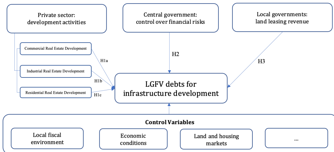
Figure 3: Analytical Framework
