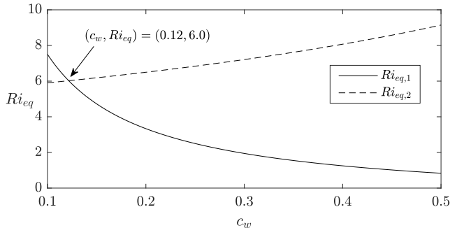
FIGURE 2. The far-field equilibrium Richardson number versus the coefficient of entrainment loss c_w for a wall plume in an unstratified environment acquired either by the expression Ri_{eq} = 5(1/c_w - 1)/6 (the solid curve, Ri_{eq,1} ) or the numerical solution of (2.9) (the dashed curve, Ri_{eq,2} ).
