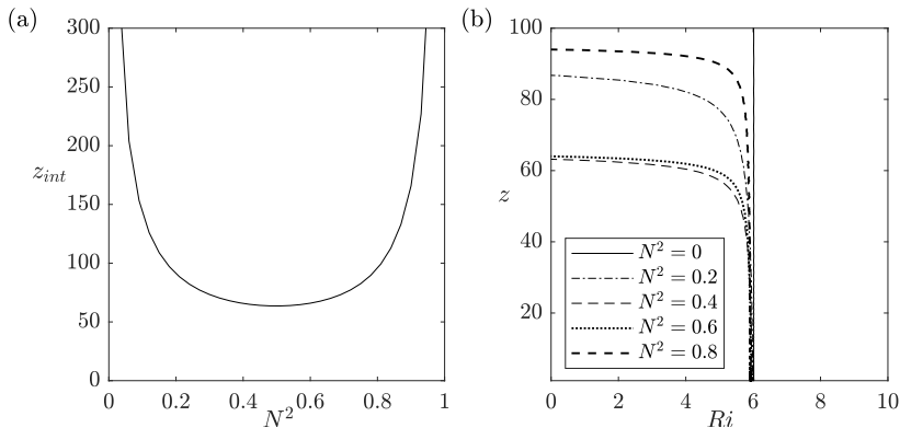
FIGURE 4. (a) Dimensionless initial discharge height versus the ambient buoyancy gradient. (b) The vertical evolution of the local Richardson number Ri = BQ^3/(2\alpha_{e,eq}M^3) .
