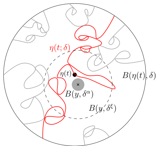
FIGURE 2. H2 existence of a ball near an excursion (depicted in red) but “far away” from other parts of the curve (depicted in grey) in the sense that any path connecting y to the grey parts of the curve must either intersect \eta(t; \delta) or exit the ball B(y, \delta^\xi) .
