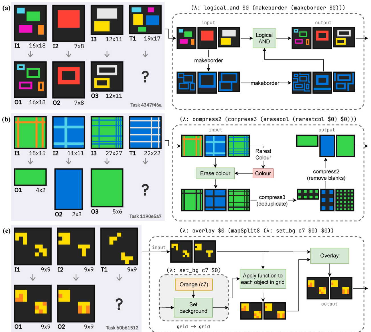
Figure 1. Three ARC tasks solved by DreamCoder (left), with the PeARL programs it generated to solve them illustrated as a computation graph (right), with intermediate outputs shown. (a) DreamCoder has no primitive to get the perimeter of objects, so it draws a border around it twice and takes the intersection with the original image. (b) Our type-system allows DreamCoder to operate on colours within images. (c) DreamCoder can use higher-order functions to apply arbitrary operations to each object in the image.
