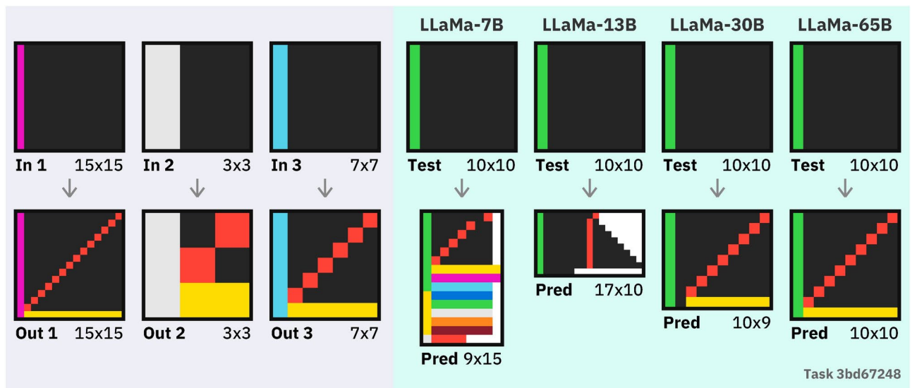
Figure 3. An example task solved by the large-language model LLaMA-65B but not by smaller models; training examples are on the left with predicted answers on the right. We see the smallest two models struggle to produce a coherent answer. The 30B model is almost correct (skipping a row and one yellow pixel), and the largest model solves the task perfectly.
