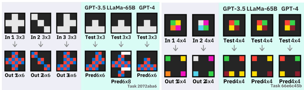
Figure 4. Two ARC-Hard tasks where only GPT-4 produced a correct solution. While the other LLMs often produce somewhat close matches on first inspection, an exactly correct solution is required to solve a task.
