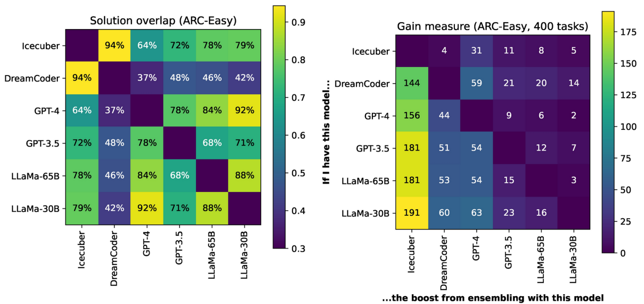
Figure 5. Comparison of the solution similarity of our systems, showing solution overlap (left panel) and gain measure (right panel) between each system: this tells us how similar the predictions are, and how much one could expect to gain by combining systems. Systems are ordered by overall performance, so the top-right triangle in the panel on the right shows the unique skills of the lesser system. The panel on the left shows that DreamCoder and GPT-4 have only 37% overlap between the tasks which they can solve.
