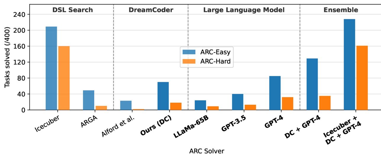
Figure 6. ARC tasks solved by each system in this work on the two available ARC datasets (see Table 3); results from this work in bold. The fully handcrafted Icecuber solver remains the best single solution, with GPT-4 obtaining slightly better performance than DreamCoder. We achieve dramatic gains by ensembling solutions. For the sake of brevity, DreamCoder is abbreviated to DC and Abstract Reasoning with Graph Abstractions 21 is abbreviated to ARGA.
