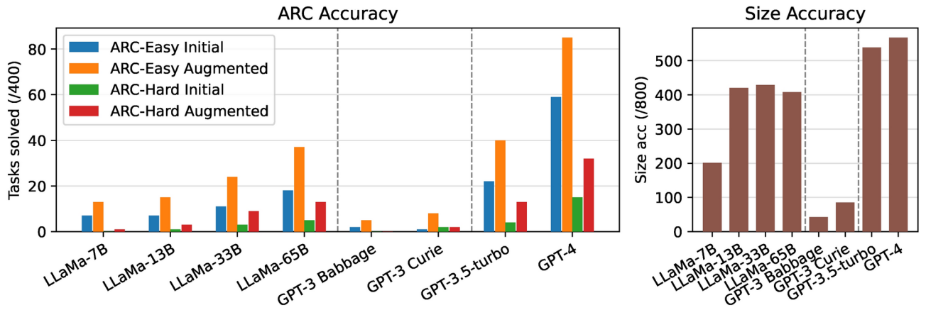
Figure 2. ARC performance of each large language model (LLM), as in Table 2. The number of correctly solved tasks is given for ARC-Easy and ARC-Hard, both on the original task and our 3-shot augmentation scheme. Size accuracy gives the number of tasks for which the LLM was able to output any grid of the correct size across both datasets.
