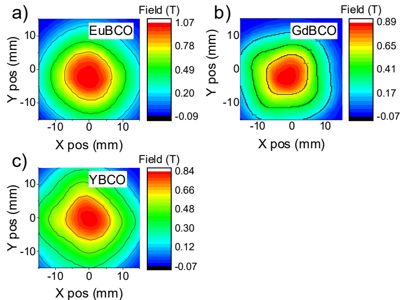
Figure 3. Trapped magnetic flux density measured using a rotating array of 18 Hall sensors 1.5 mm above top surface of a) EuBCO, b) GdBCO and c) YBCO single-grains using FCM at 77 K. The EuBCO sample exhibits the highest trapped field of 1.26 T, as measured by a handheld gaussmeter on its top surface, and also the most symmetric field distribution.
