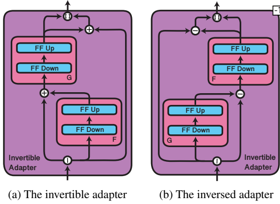
Figure 2: The invertible adapter (a) and its inverse (b). The input is split and transformed by projections F and G , which are coupled in an alternating fashion. || indicates the splitting of the input vector, and [] indicates the concatenation of two vectors. + and - indicate element-wise addition and subtraction, respectively.
