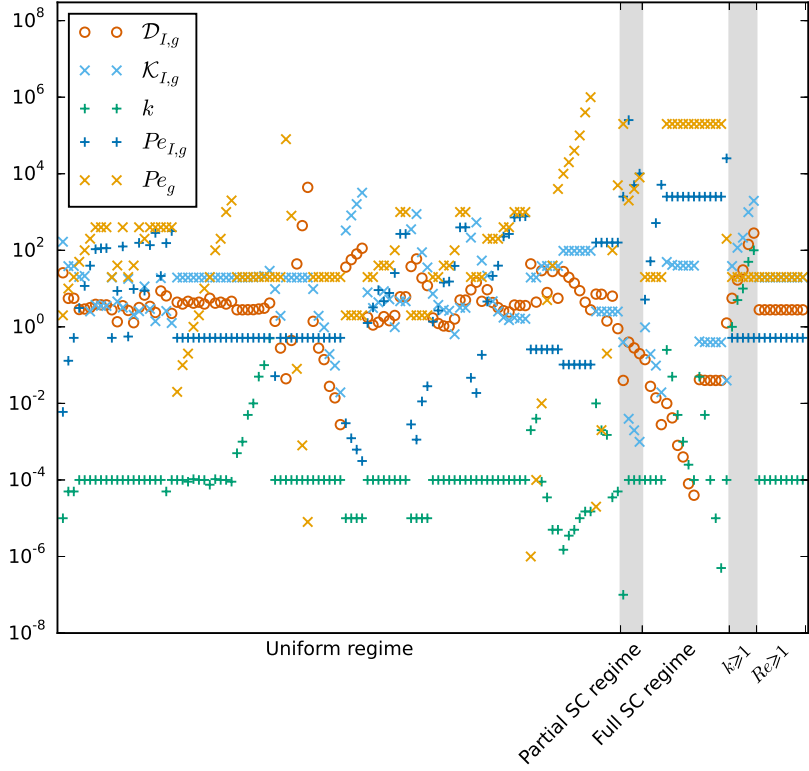
Figure 8. Variation of some of the characteristic non-dimensional numbers used in our 137 numerical simulations depending on the regime. The non-dimensional number K_{I,g} = Bi_g(1 + k)/F_0 the ratio of the adsorption{desorption} kinetics flux to the advective flux at the interface. The parameter D_{I,g} = \chi_g(1 + k)/(F_0 Pe_g)^{1/2} is the ratio of the transverse diffusive flux through the diffusive boundary layer to the advective flux at the interface. The function F_0 = F(g, \phi, x = 0) is related to the interfacial slip velocity following (67).
