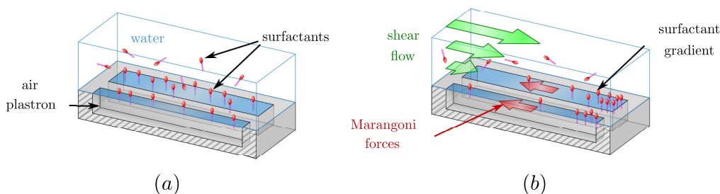
Figure 1. Schematic illustrating the impact of surfactants above a superhydrophobic surface (SHS) made of longitudinal rectangular grating. (a) Surfactants present in water adsorb at the air-water interface of the gratings. (b) In the presence of an external flow, surfactants distribute in gradients between stagnation points, yielding a Marangoni stress opposing the flow.
