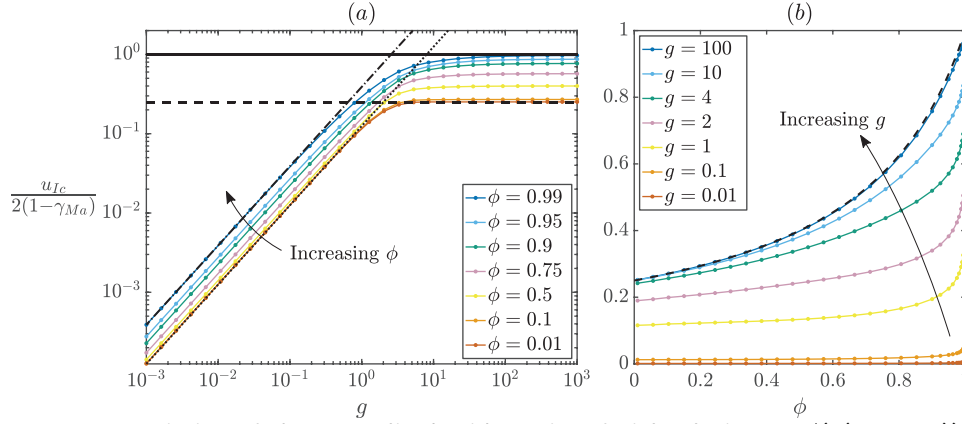
Figure 3. Variation of the normalised mid-gap interfacial velocity, u_{Ic}/(2(1-\gamma_{Ma})) = F(g, \phi, x=0) = F_0(g, \phi) (see (67) and text), as a function of: (a) the non-dimensional interfacial length g , for different non-dimensional gas fraction from \phi = 0.01 to 0.99 (shown with different colors, see legend); (b) the gas fraction \phi , for various interfacial lengths g (shown with different colors, see legend). The implicit function F_0(g, \phi) has been computed by solving the linear system (57) with N = 500 , except in the more demanding cases of 0.01 < \phi < 0.1 ( N = 2,500 ), 0.99 < \phi < 1 ( N = 2,500 ) and 0 < \phi < 0.01 ( N = 15,000 ). In (a) the black dotted line is plotted using (69) for \phi = 1 and g = 1 , the black dot-dashed line is plotted using (120) for g = 1 and \phi = 0.99 , and the black dashed line is plotted using (70) for \phi = 1 and g \gg 1 . The black solid line corresponds to the maximum asymptotic value for \phi \rightarrow 1 : u_{Ic} \rightarrow u_u(y=1) = 2(1-\gamma_{Ma}) (see (72)). In (b), the black dashed line has been plotted using the asymptotic trend (73) for g \rightarrow 1 (see also appendix C).
